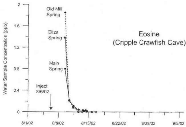
Figure 7: Breakthrough curves of sodium fluorescein and eosine at Barton Springs.
