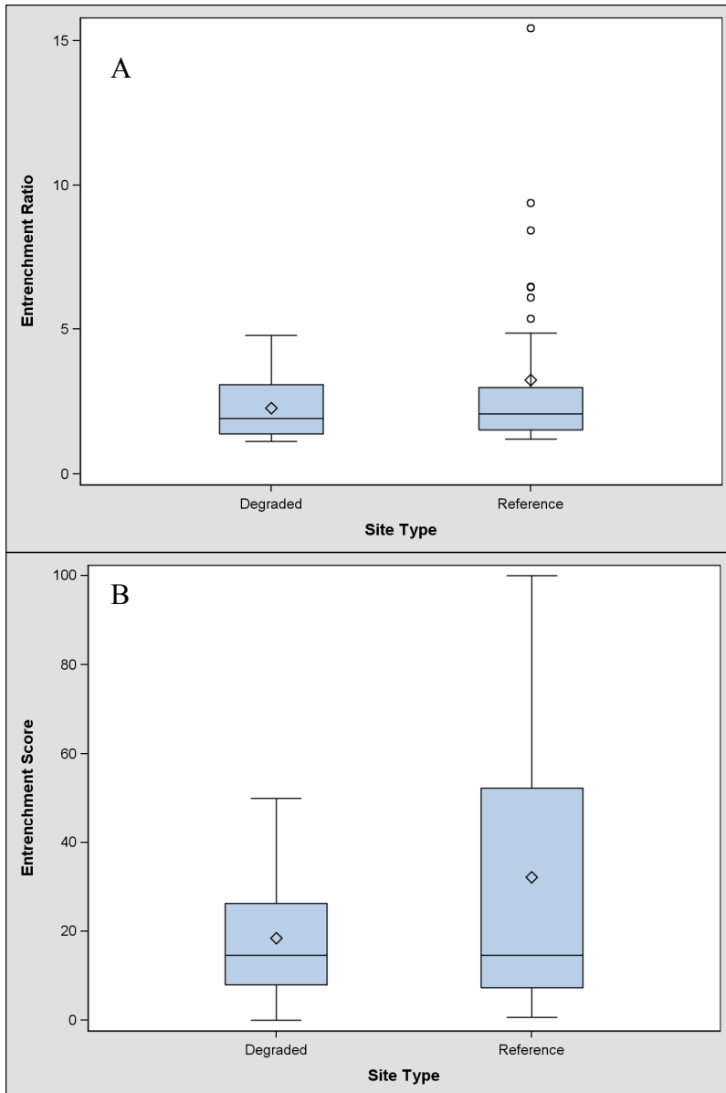
Figure 7: Boxplot of A) the raw entrenchment ratio and B) entrenchment scores at degraded and reference sites. Means are diamonds, medians are horizontal lines, and outliers are circles.
