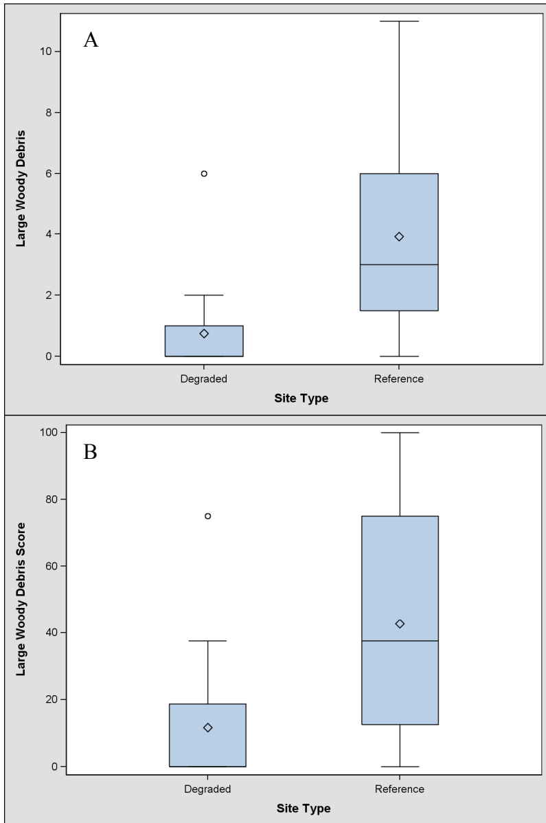
Figure 6: Boxplot of A) raw large woody debris counts and B) large woody debris scores at degraded and reference sites. Means are diamonds, medians are horizontal lines, and outliers are circles.
