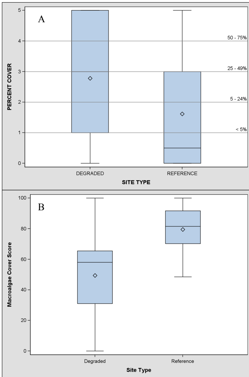
Figure 2: Boxplot of A) categorical macroalgae percent cover based on the zig-zag collection method B) macroalgae cover scores for degraded and reference sites. Percent cover classifications include 0= none, 1= <5%, 2= 5-24%, 3= 25-49%, 4= 50-75%, 5= >75%. Diamonds are means and lines are medians.
