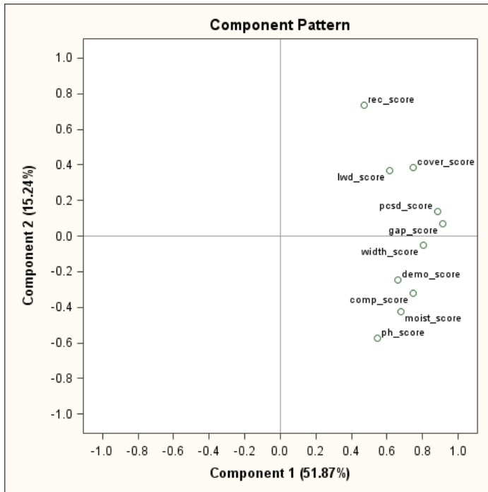
Figure 16: Principal Component Analysis of the functional parameters collected for the Riparian Functional Assessment.
