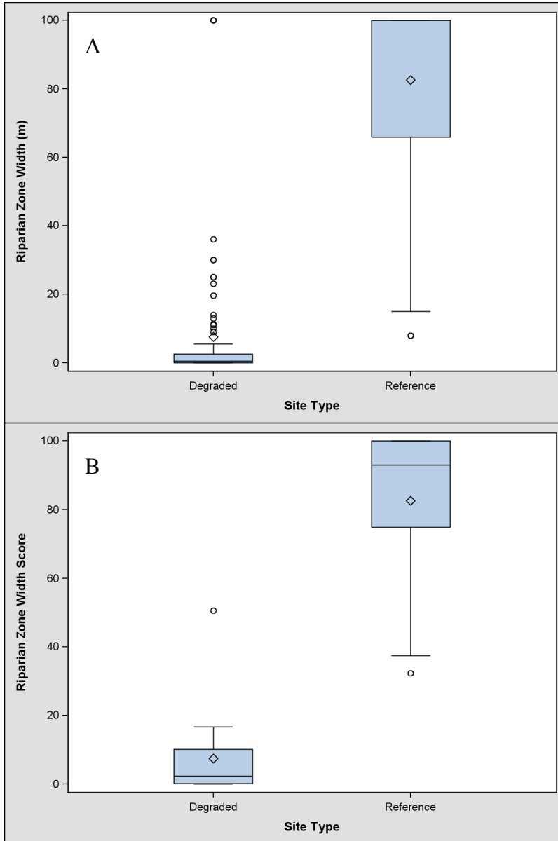
Figure 13: Boxplots of A) riparian zone width and B) riparian zone width scores at degraded and reference sites. Means are diamonds, medians are horizontal lines, and outliers are circles.
