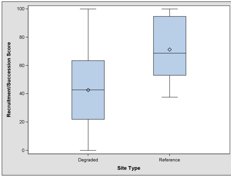
Figure 15: Boxplot of recruitment/succession scores at degraded and reference sites. Means are diamonds, medians are horizontal lines, and outliers are circles.
