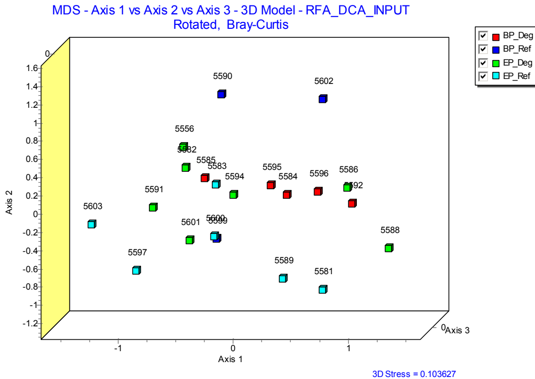
Figure 3: Non-metric Multidimensional Scaling (nMDS) ordination of diatom community structures. Legend labels are as follows: BP_Deg = Blackland Prairie Degraded, BP_Ref = Blackland Prairie Reference, EP_Deg = Edward's Plateau Degraded, EP_Ref = Edward's Plateau Reference.
