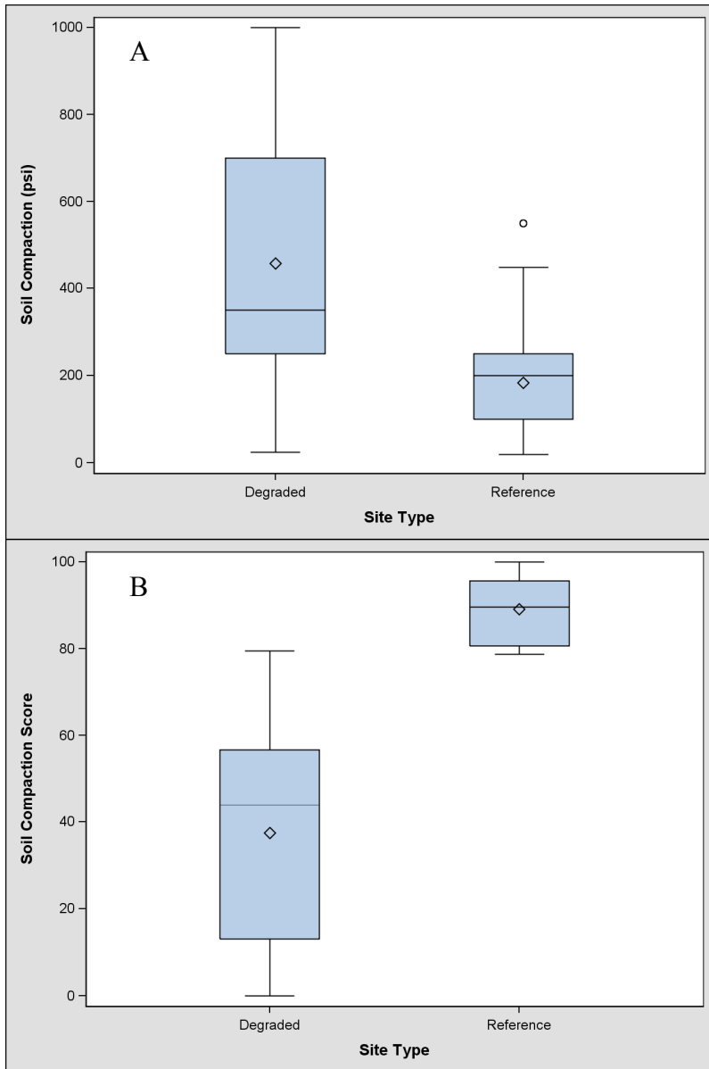
Figure 9: Boxplot of A) soil compaction and B) soil compaction scores at degraded and reference sites. Means are diamonds, medians are horizontal lines, and outliers are circles.
