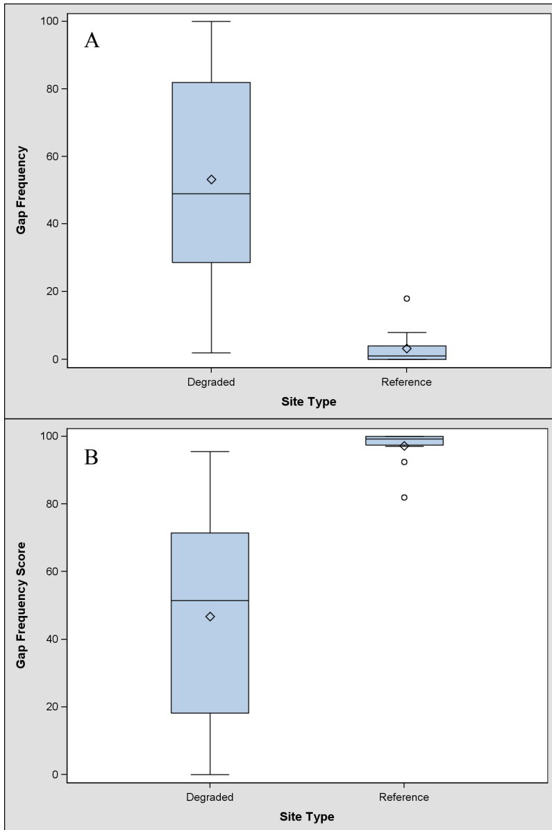
Figure 4: Boxplot of A) raw gap frequency and B) gap frequency scores at degraded and reference sites. Means are diamonds, medians are horizontal lines, and outliers are circles.
