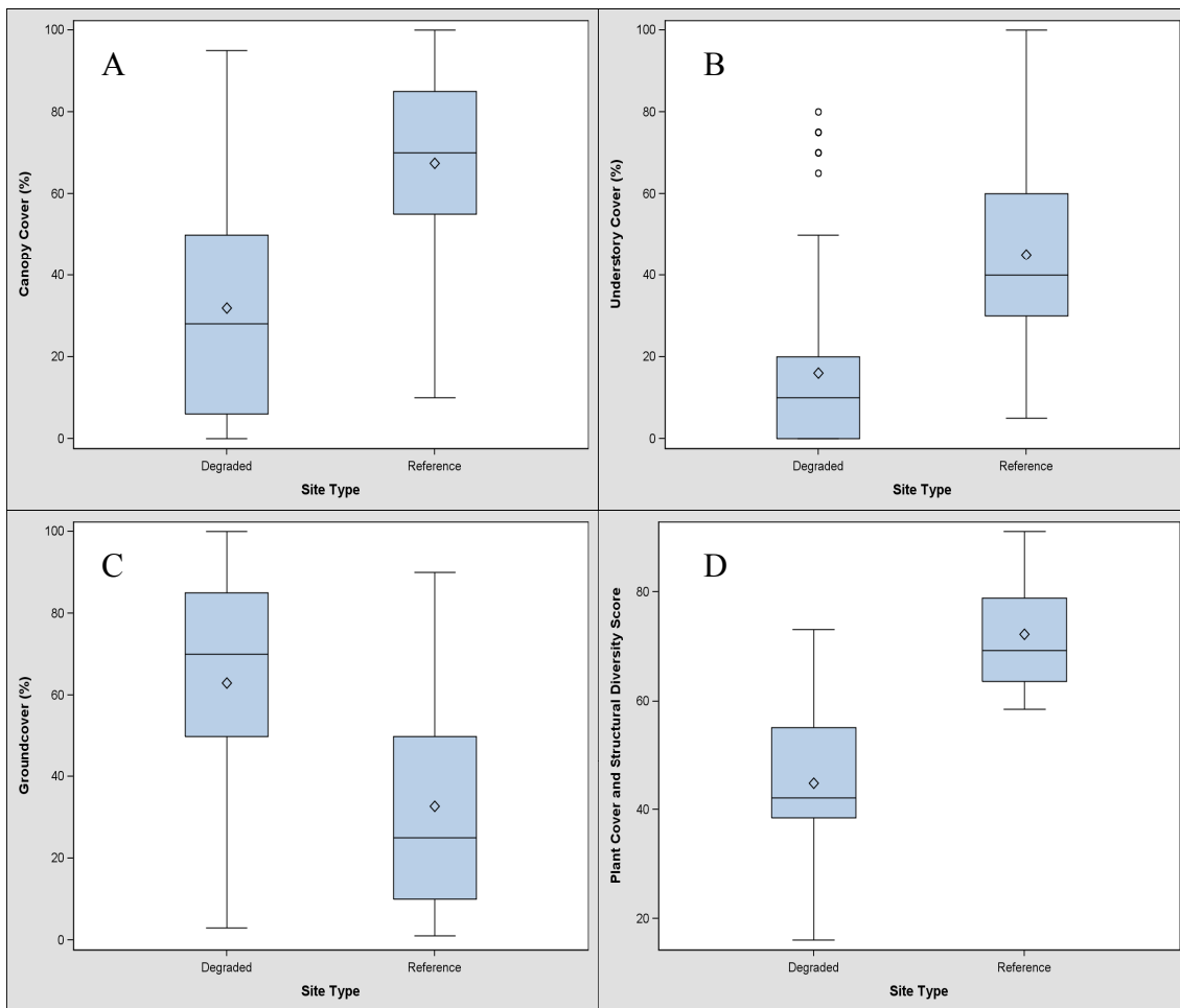
Figure 12: Boxplots of A) percent canopy cover, B) percent understory cover, C) percent groundcover, and D) plant cover and structural diversity scores at degraded and reference sites. Means are diamonds, medians are horizontal lines, and outliers are circles.
