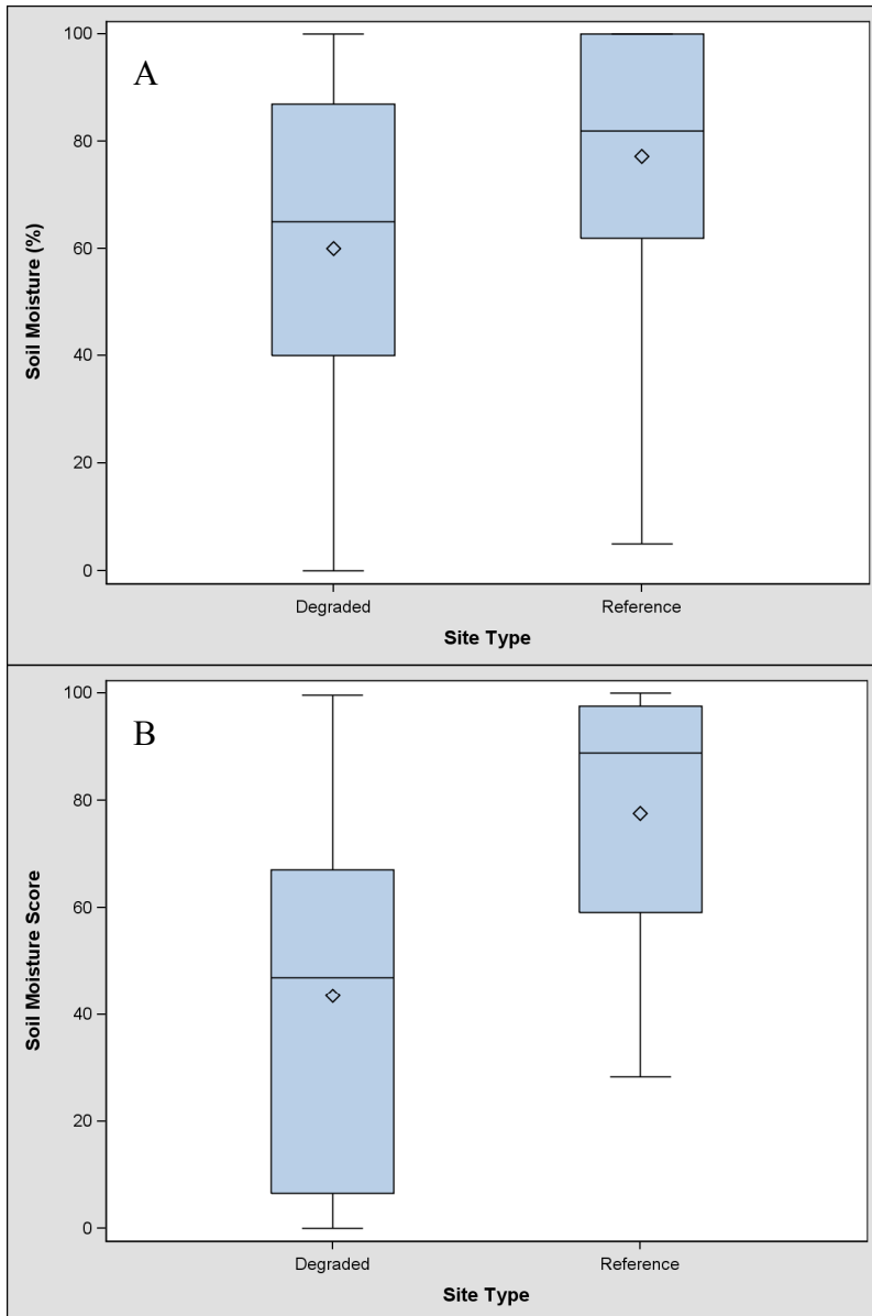
Figure 10: Boxplot of A) soil moisture and B) soil moisture scores at degraded and reference sites. Means are diamonds, medians are horizontal lines, and outliers are circles.
