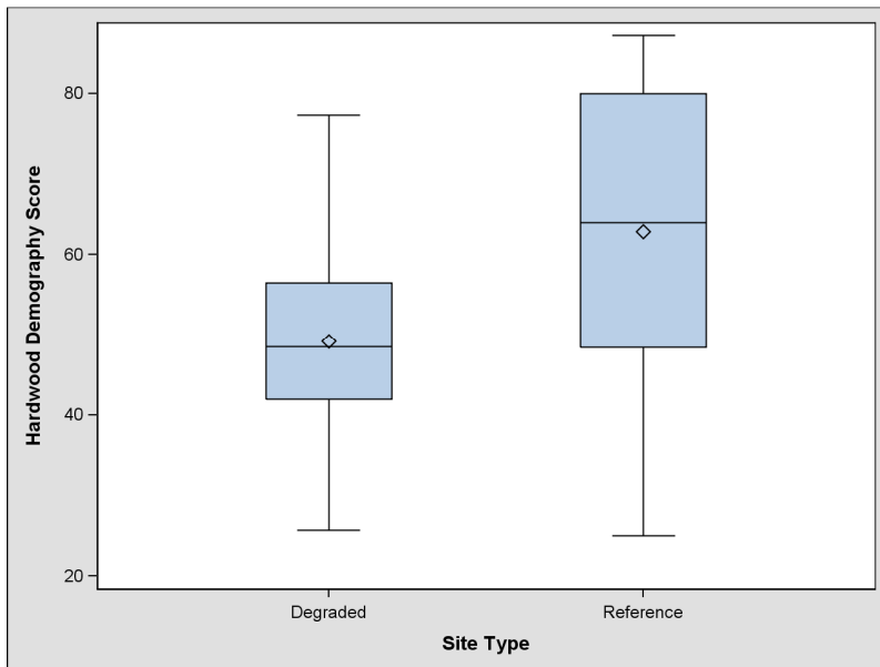
Figure 14: Boxplot of hardwood demography scores at degraded and reference sites. Means are diamonds, medians are horizontal lines, and outliers are circles.
