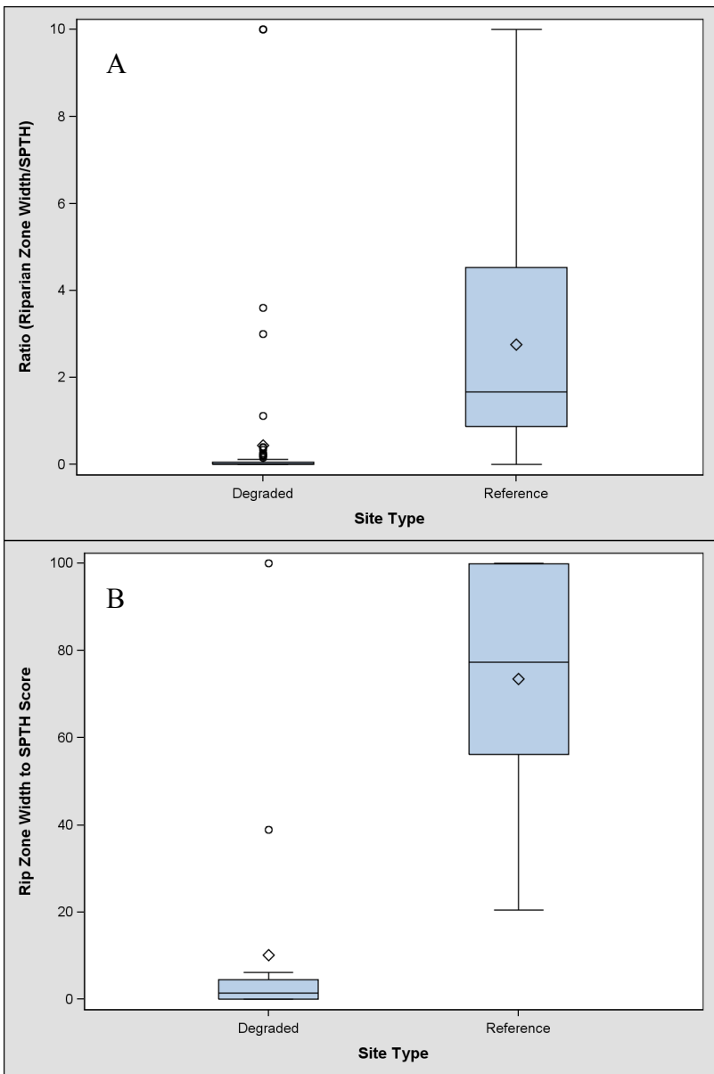
Figure 14: Boxplots of A) riparian zone width to SPTH and B) riparian zone width to SPTH scores at degraded and reference sites. Means are diamonds, medians are horizontal lines, and outliers are circles.
