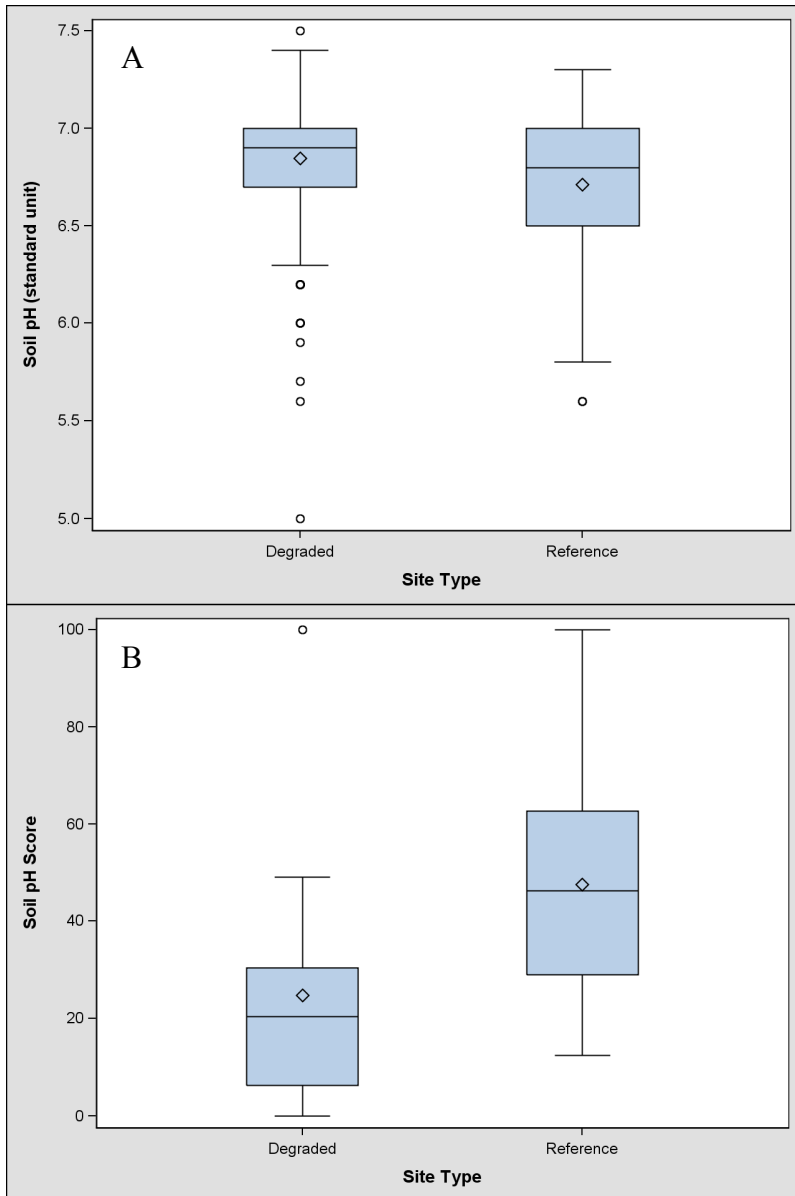
Figure 11: Boxplot of A) soil pH and B) soil pH scores at degraded and reference sites. Means are diamonds, medians are horizontal lines, and outliers are circles.
