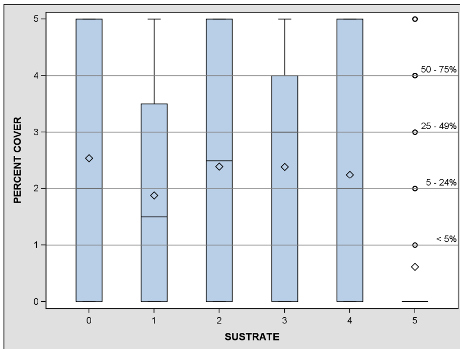
Figure 1: Boxplot of macroalgae cover for various types of substrate within the study. Percent cover classifications include 0= none, 1= <5%, 2= 5-24%, 3= 25-49%, 4= 50-75%, 5= >75%. Diamonds are means and lines are medians.
