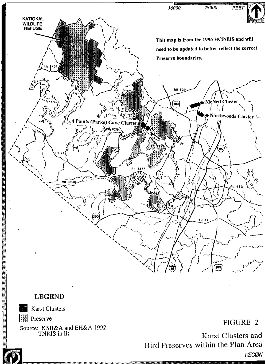
Figure 2. Karst Clusters
