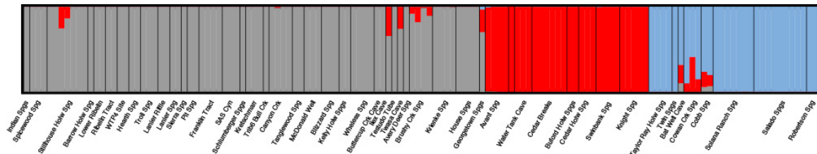
Figure 3. Structure analysis ( K = 3 ) of Eurycea from north of the Colorado River, based on 75,296 loci. Vertical bars represent individuals; black lines separate populations. The three colors represent the three major genetic divisions, and correspond to populations of the three described species. Gray = E. tonkawae ; Red = E. naufragia ; Blue = E. chisholmensis .
