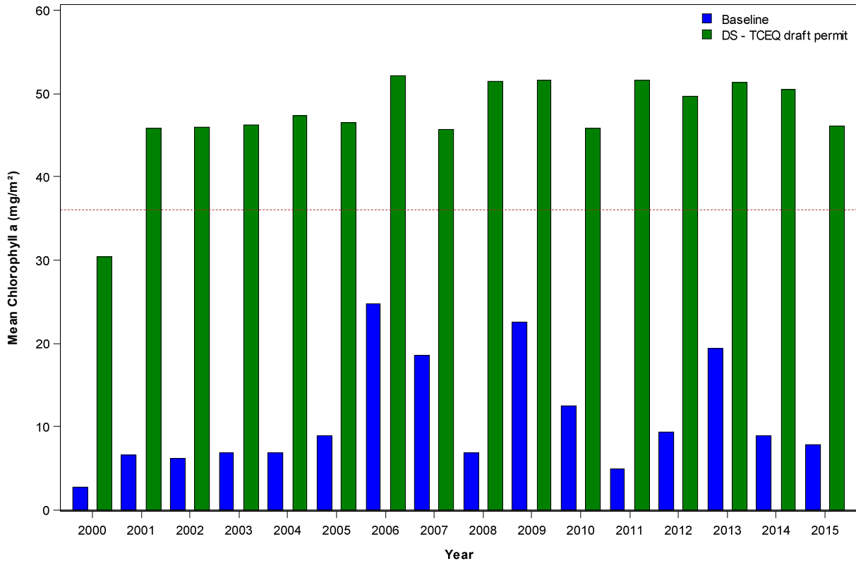
Figure 8: Annual mean benthic chlorophyll a (mg/m 2 ) from modeled data on Onion Creek at a distance of 200 m (656 ft.) from where the City of Dripping Springs WWTP effluent would enter Onion Creek. Means for the Baseline scenario where no effluent is discharged are blue while means for the Discharge scenario are green. Onion Creek would be considered in an oligotrophic state in the Baseline scenario but in a mesotrophic state in the Discharge scenario using the threshold proposed by Dodds (2006).
