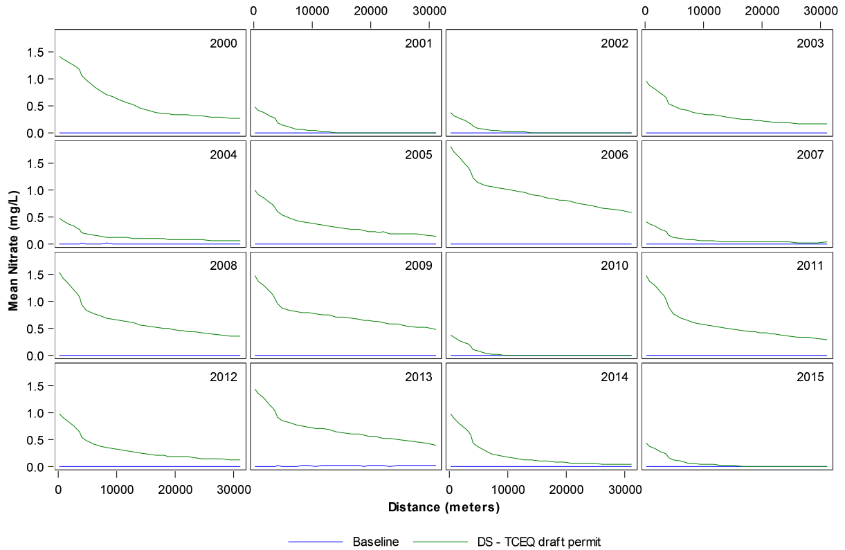
Figure 10: Annual mean nitrate as nitrogen (NO 3 -N) against distance (meters) from the WWTP discharge. Blue lines indicate NO 3 -N concentrations without the discharge while green lines indicate NO 3 -N concentrations with the discharge. In the presence of the WWTP discharge, annual mean concentrations of NO 3 -N in Onion Creek just downstream of the introduction to the treated effluent are predicted to be approximately 60 to 200 times the annual mean baseline concentrations depending on the year.
