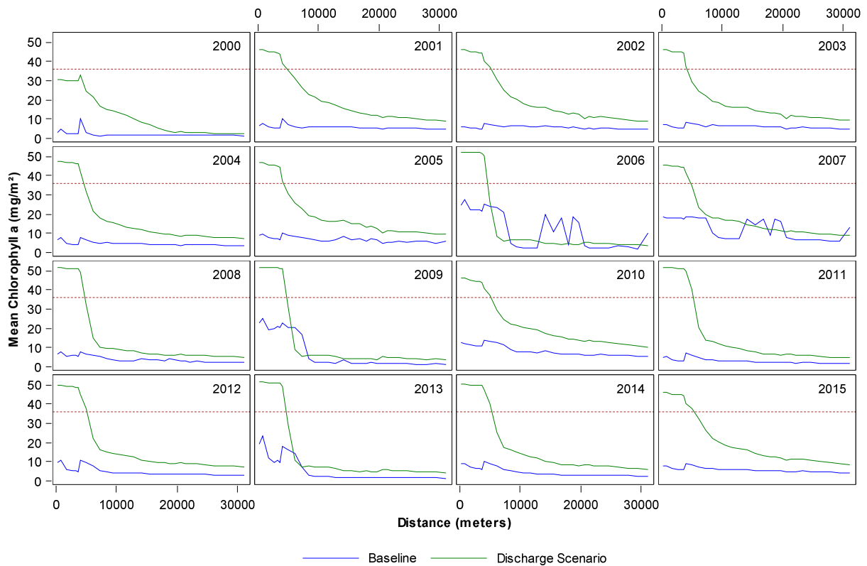
Figure 9: Annual mean chlorophyll a against distance (meters) from the WWTP discharge. Blue lines indicate chlorophyll a concentrations without the discharge while green lines indicate chlorophyll a concentrations with the discharge. The brown line indicates the threshold between oligotrophic and mesotrophic status based on benthic chlorophyll a (36 mg/m 2 ) proposed by Dodds (2006). In the presence of the WWTP discharge, Onion Creek will degrade to a mesotrophic status at the point of discharge and remain in that status for 4,067 to 4,871 m (2.53 to 3.03 miles) depending on the year.
