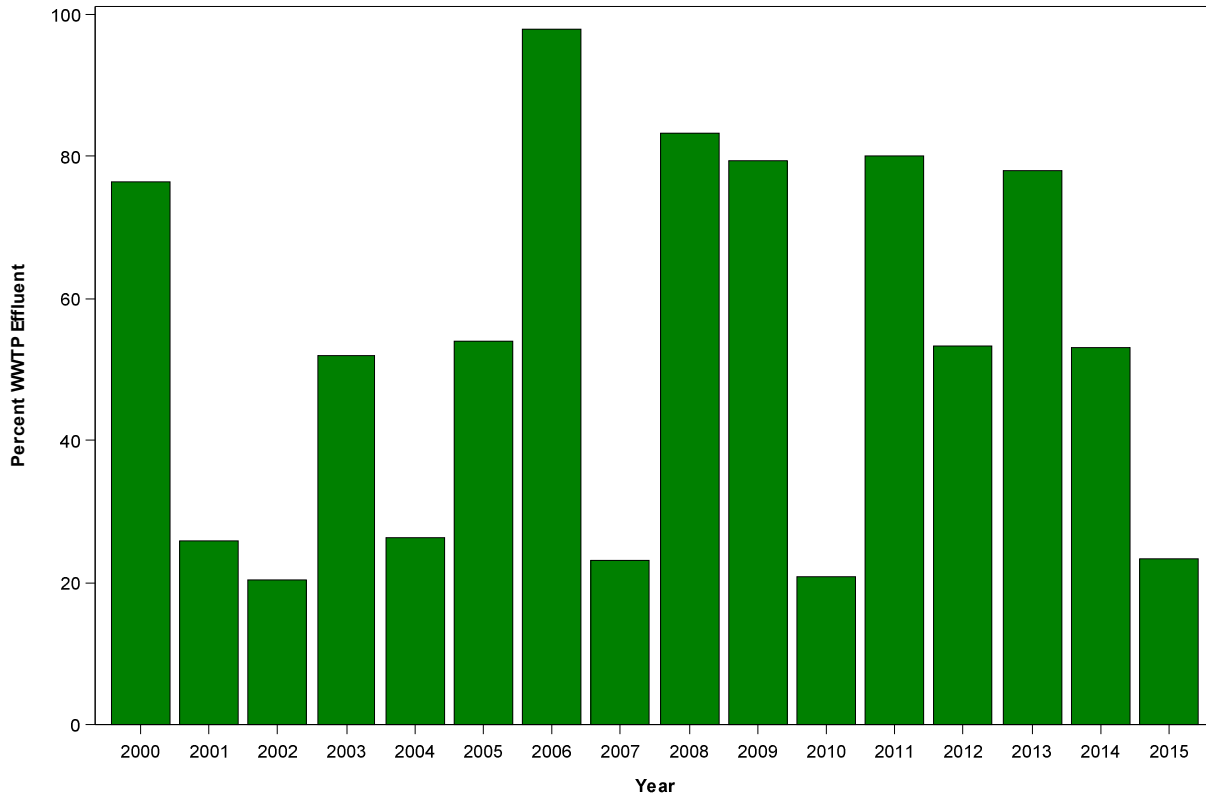
Figure 11: Annual mean percentage of treated wastewater to the Onion Creek flow at a distance of 200 m (656 ft.) from where the Dripping Springs WWTP effluent would enter Onion Creek. Means range from less than 20% to approximately 98% it an extremely dry year.
