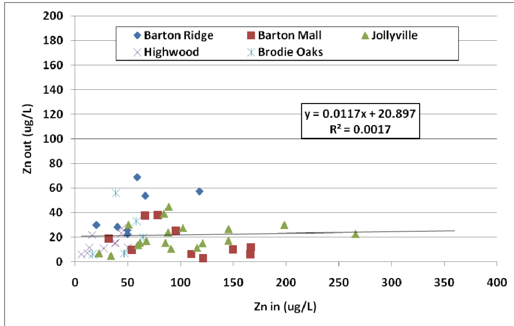
Figure 92 Relationship between Zn Influent and Effluent Concentrations
