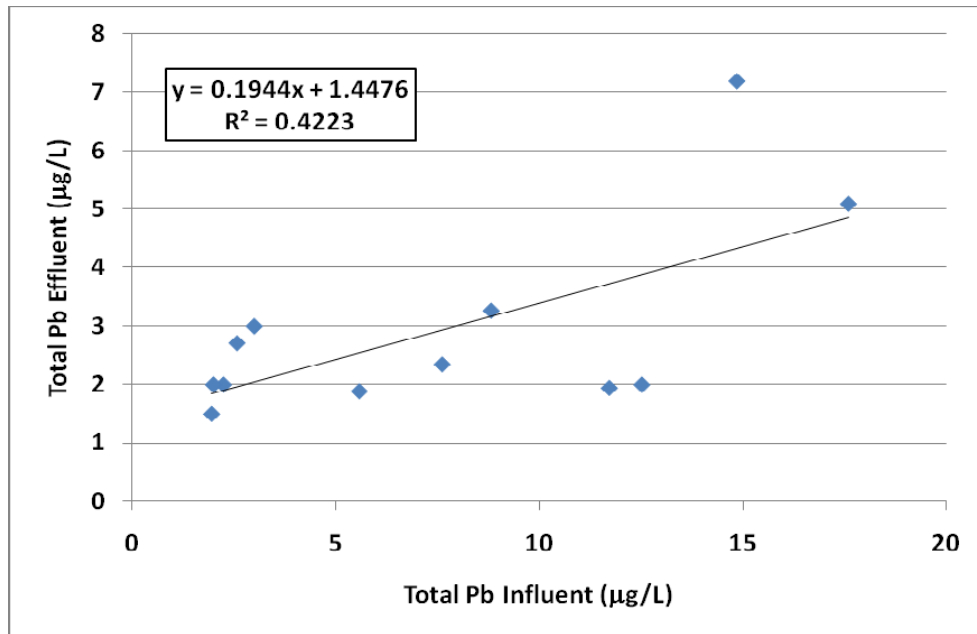
Figure 110 Relationship between Pb Influent and Effluent Concentrations Highwood
