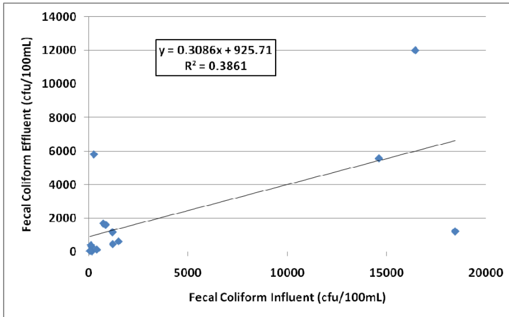
Figure 55 Relationship between FC Influent and Effluent Concentrations Jollyville
