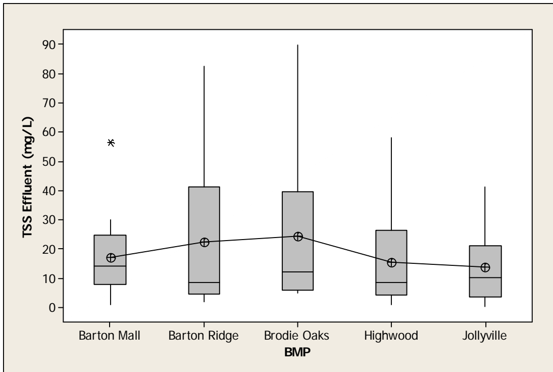
Figure 6 Boxplot of TSS Discharge Concentrations (all data)
