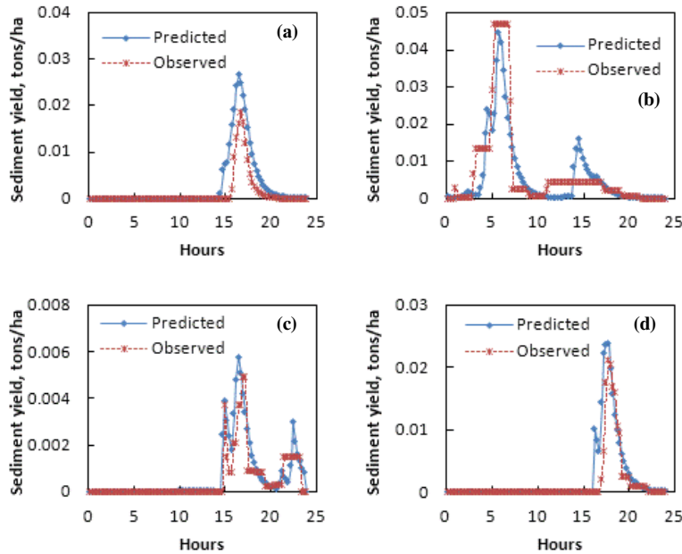
Figure 3. Calibrated sediment yield at the Y-2 outlet for events on (a) 8 March 2001, (b) 16 December 2001, (c) 21 October 2002, and (d) 30 December 2002.
