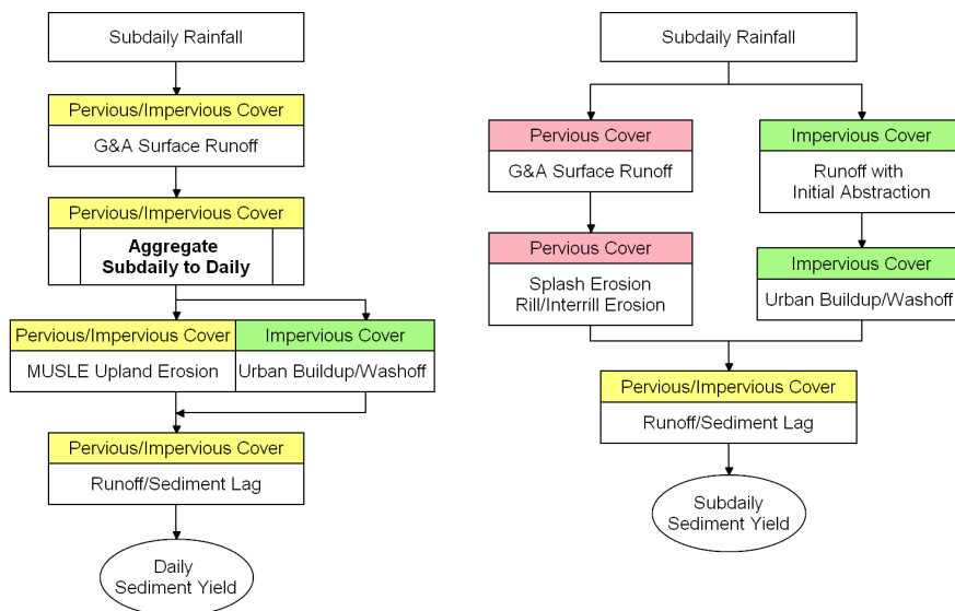
Figure 1. Schematic of sub-daily erosion processes (right) compared to daily erosion processes in SWAT2005 (left).
