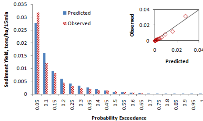
Figure 4. Exceedance probabilities for measured sediment yield data from watershed Y-2 and SWAT sub-daily predictions.
