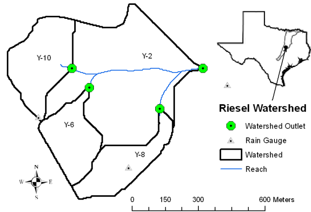
Figure 2. Experimental watersheds and rain gauges at the USDA-ARS Grassland, Soil and Water Research Laboratory near Riesel, Texas.
