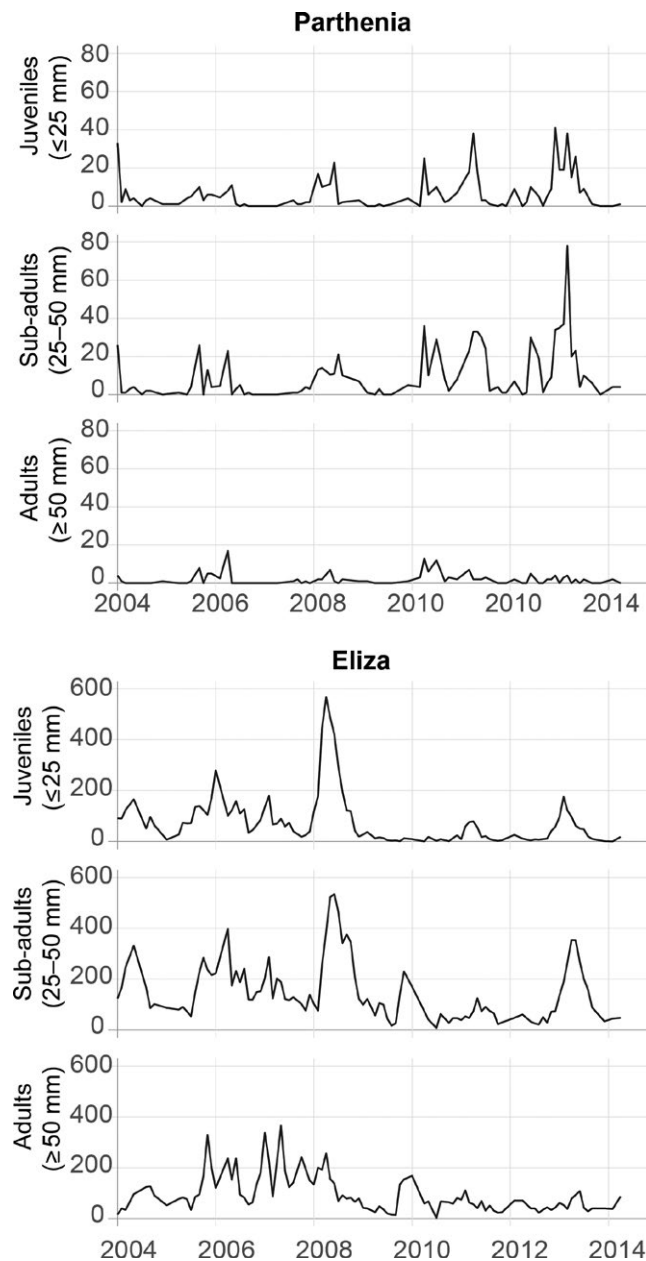
FIGURE 2 Time series of counts of E. sosorum by size class from 2004 to 2014 from Parthenia and Eliza springs. Data from each site are plotted to different y-axes
