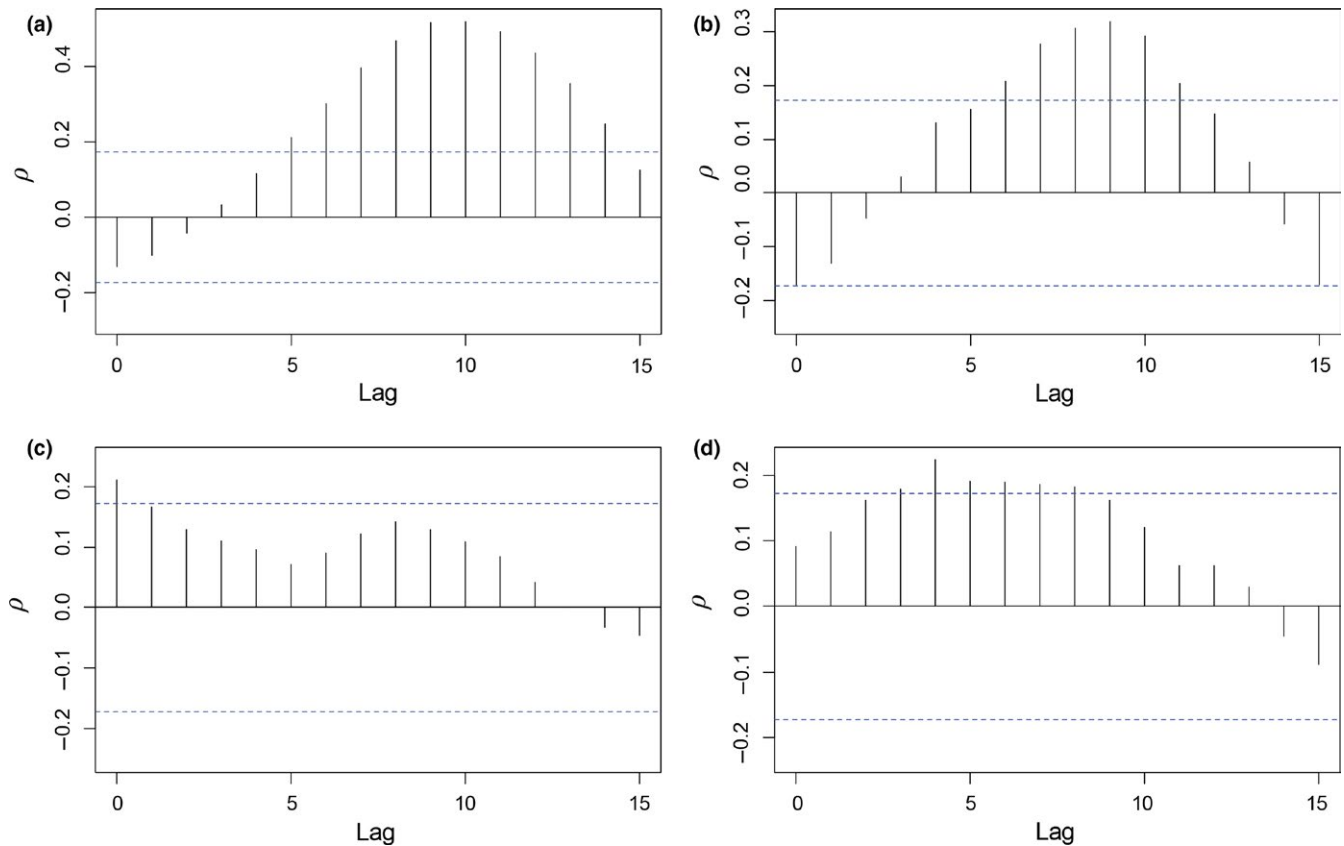
FIGURE 3 Cross-correlation between counts of E. sisorum and mean monthly discharge of Barton Springs at lags k = 0 –15 months. (a) Juvenile ( \leq 25 mm TL) abundance at Eliza; (b) Juvenile abundance at Parthenia; (c) Adult ( \geq 50 mm TL) abundance at Eliza; (d) Adult abundance at Parthenia. Dashed lines represent 95% confidence limits (calculated at lag k = 1 )
