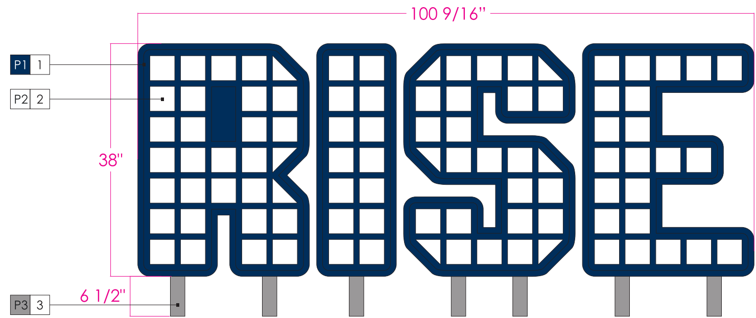
face view scale: 3/4" = 1'
