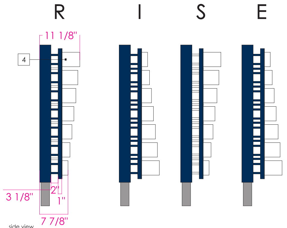
side view scale: 3/4" = 1'
