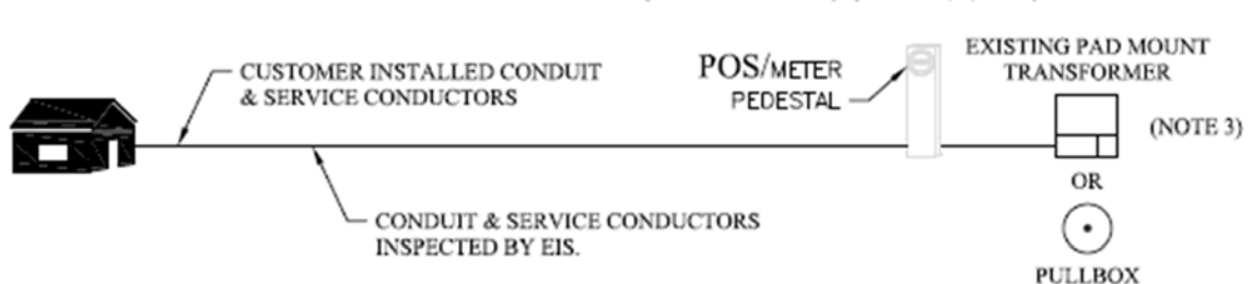
Figure 1-37B Residential Underground Service Lateral Responsibilities
