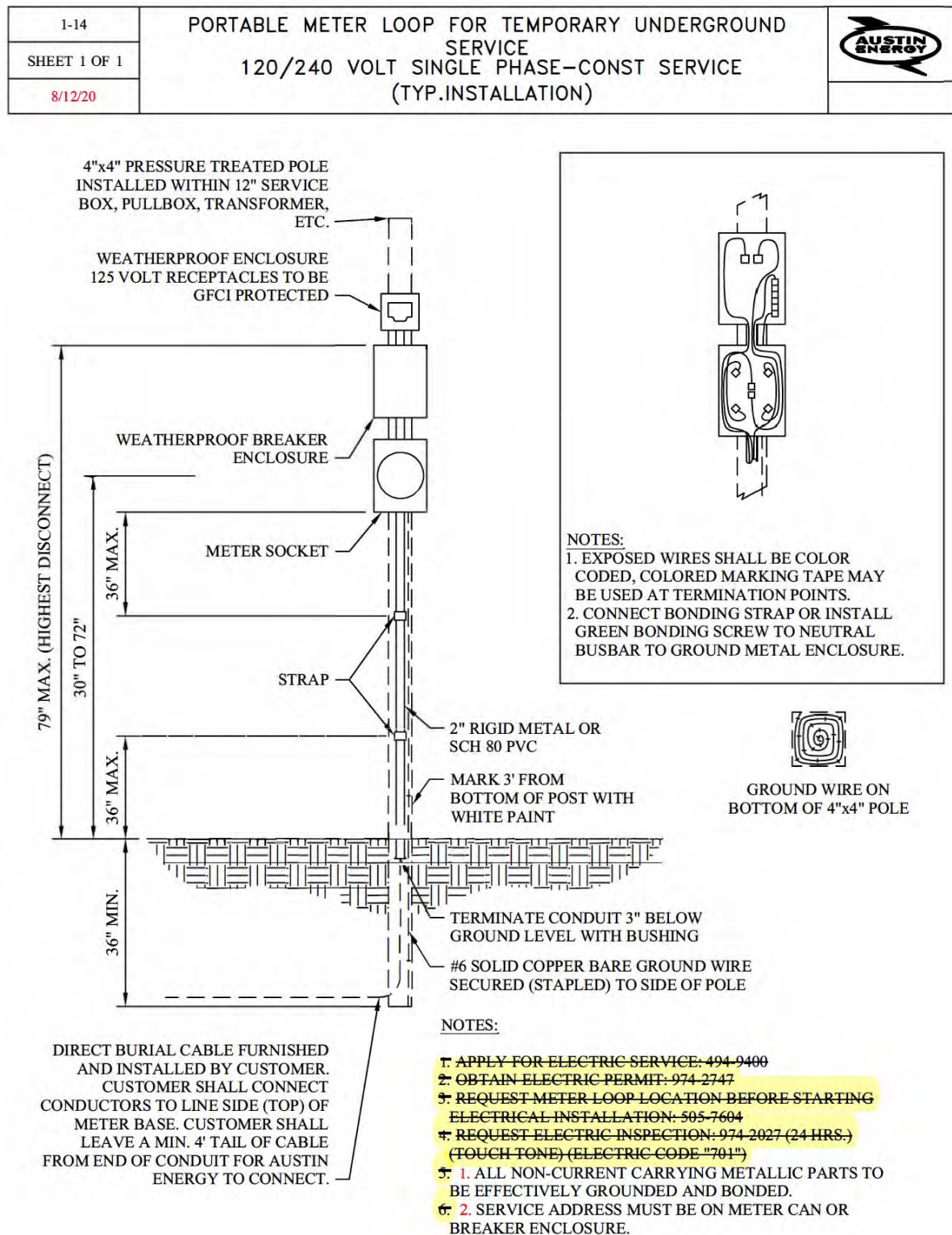
Figure 1-14. Portable Meter Loop for Temporary Underground Construction Service (Typical Installation)
