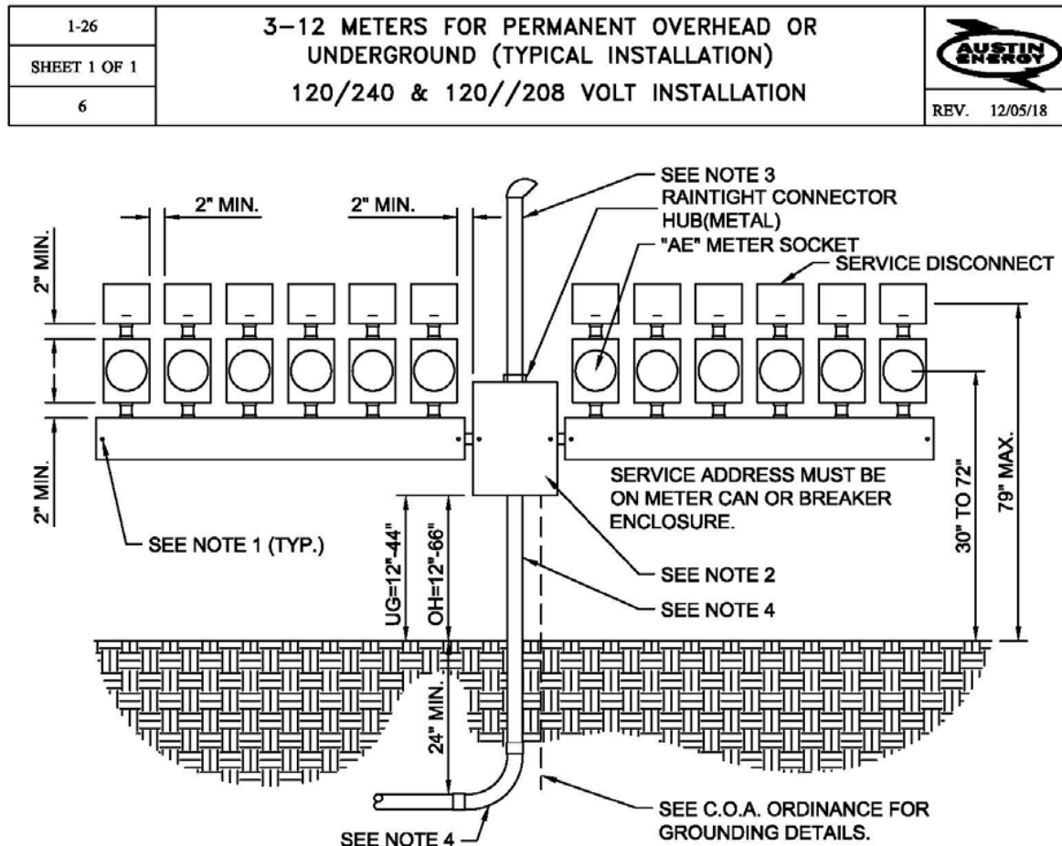
Figure 1-26. 3 to 12 Meters for Permanent Overhead or Underground Installation (Typical Installation)
