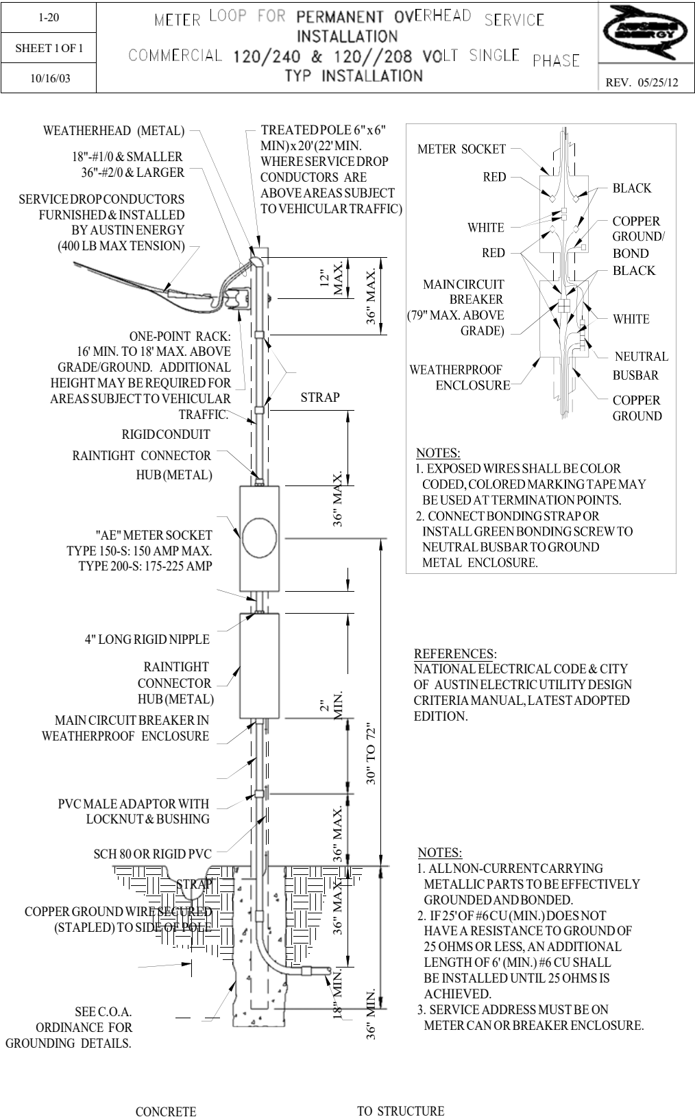
Figure 1-20. Meter Loop for Permanent Overhead Service Installation (Commercial – Typical Installation)
