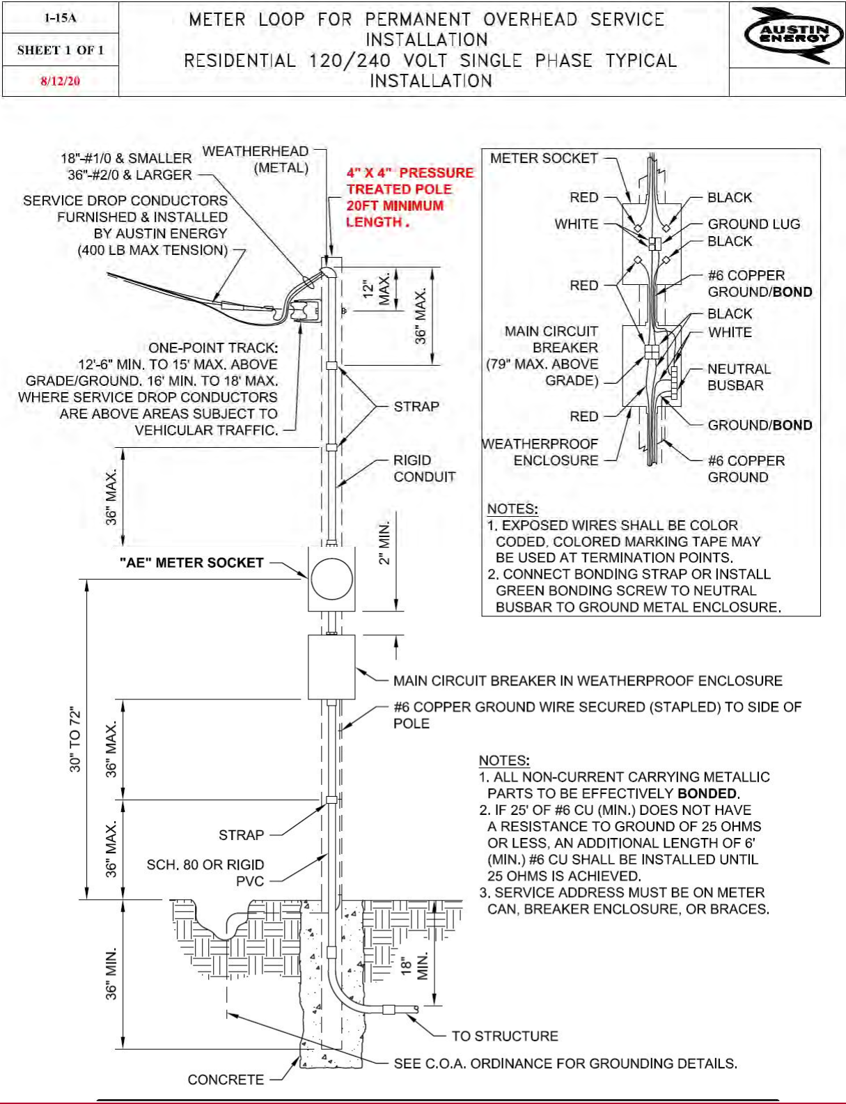
Figure 1-15A. Meter Loop for Permanent Overhead Service Installation ( Residential- Typical Residential Installation)
