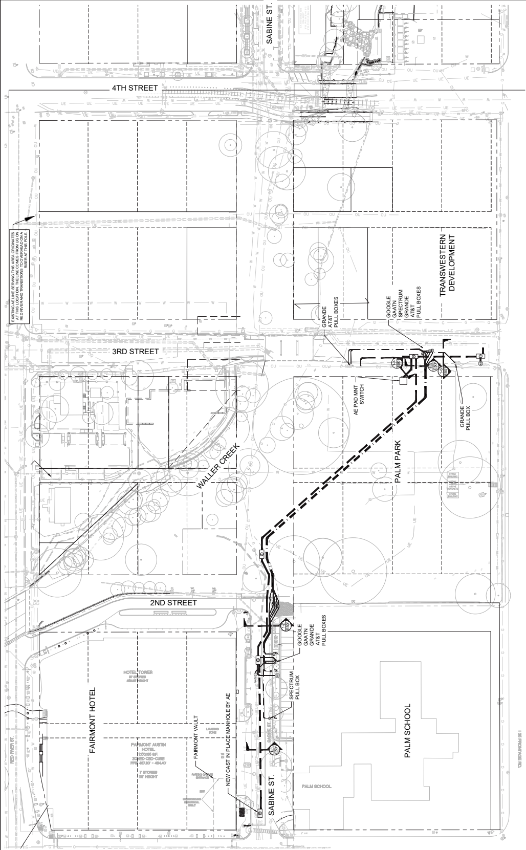
1 UNDERGROUND DUCT-BANK OVERALL PLAN - PALM PARK UTILITY RELOCATION - PHASE 1
