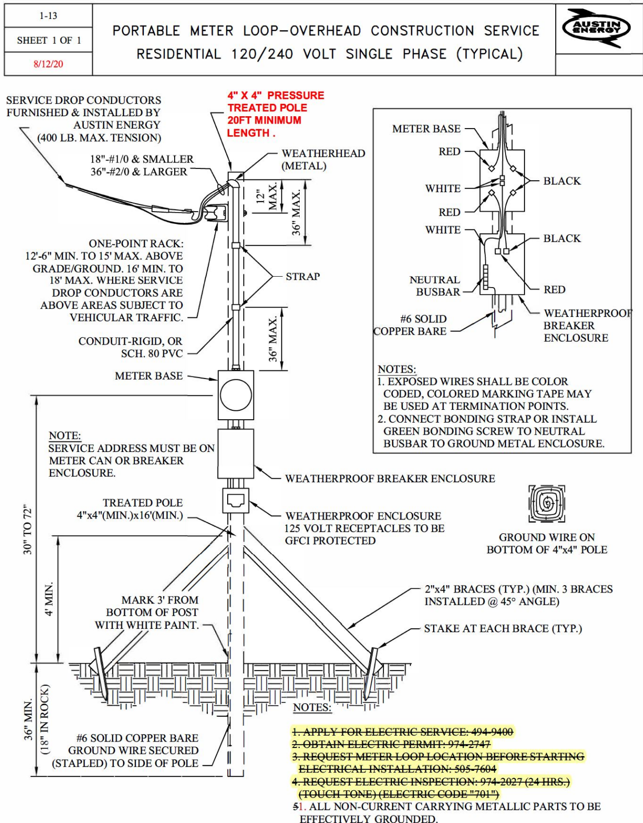
Figure 1-13. Portable Meter Loop for Temporary Overhead Construction Service (Typical Installation)
