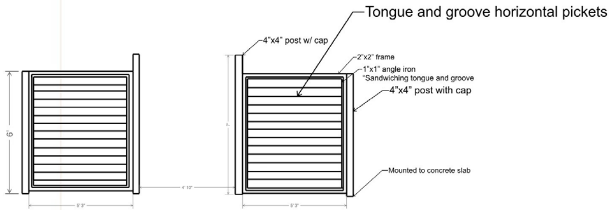
Fence design
