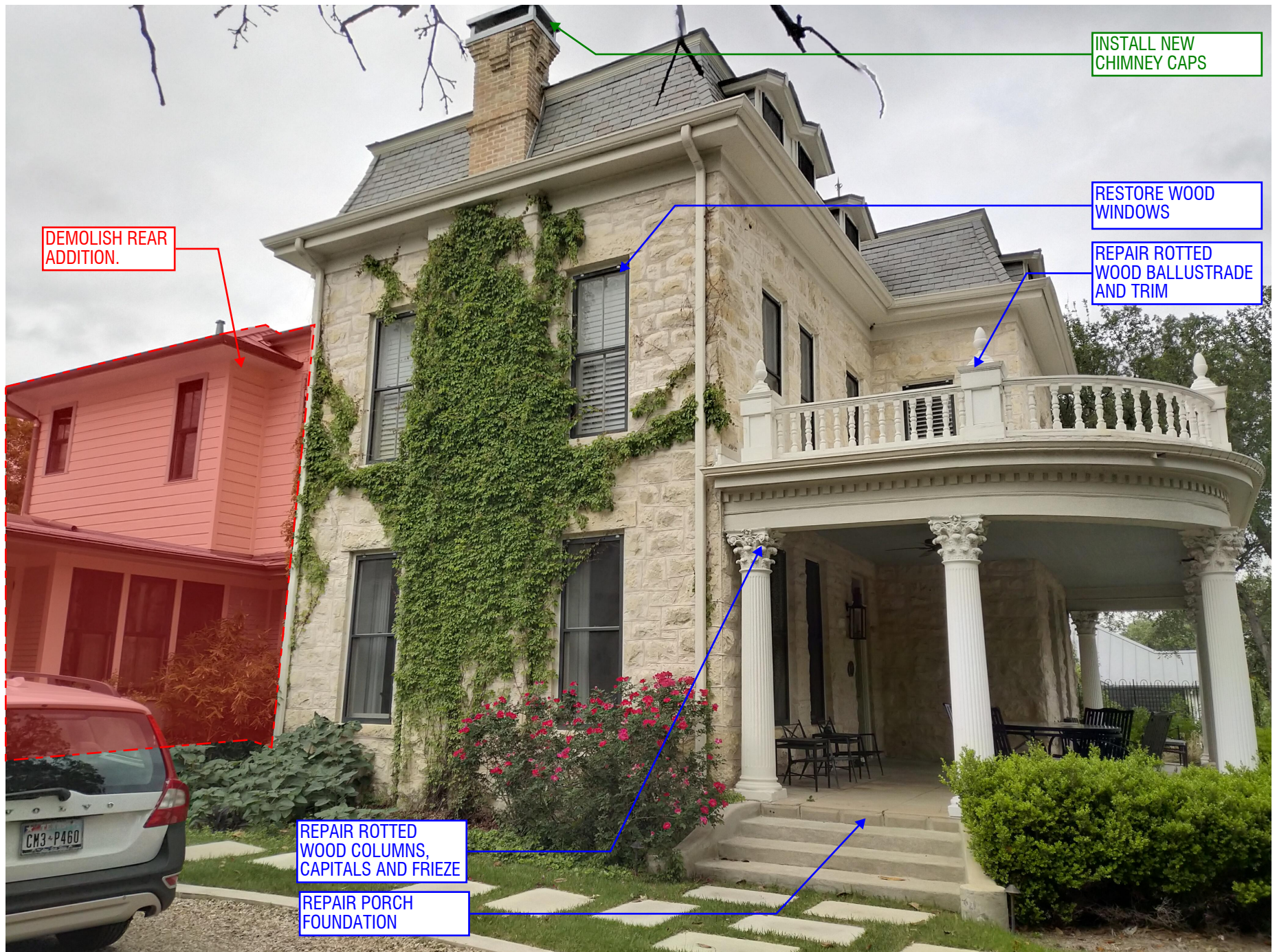
WEST FACADE
