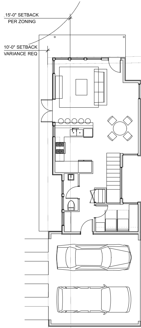
2 MAIN UNIT, 1ST FLOOR Scale: 1/8" = 1'-0"
