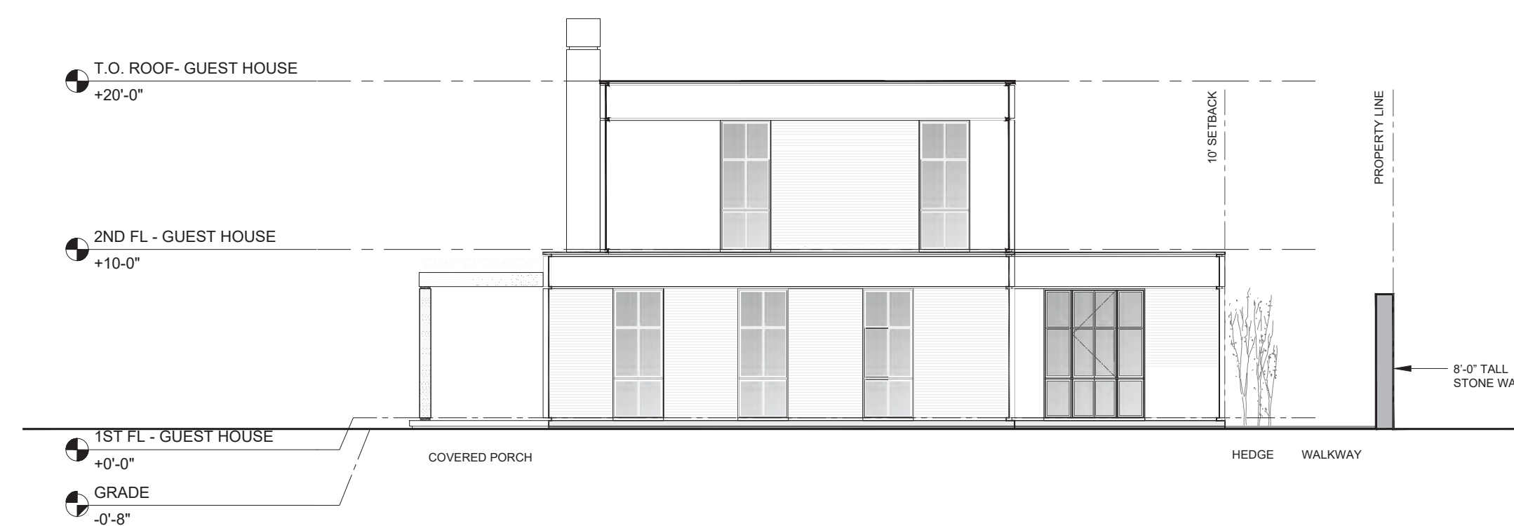
NORTH ELEVATION
