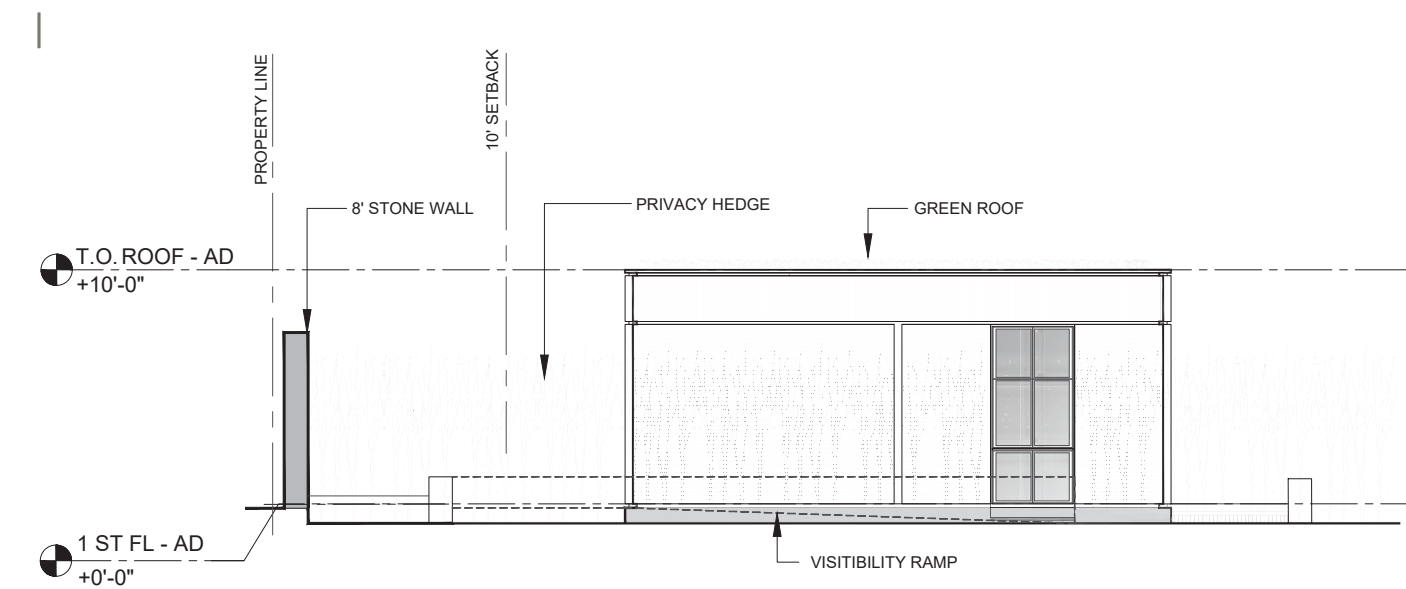
SOUTH ELEVATION
