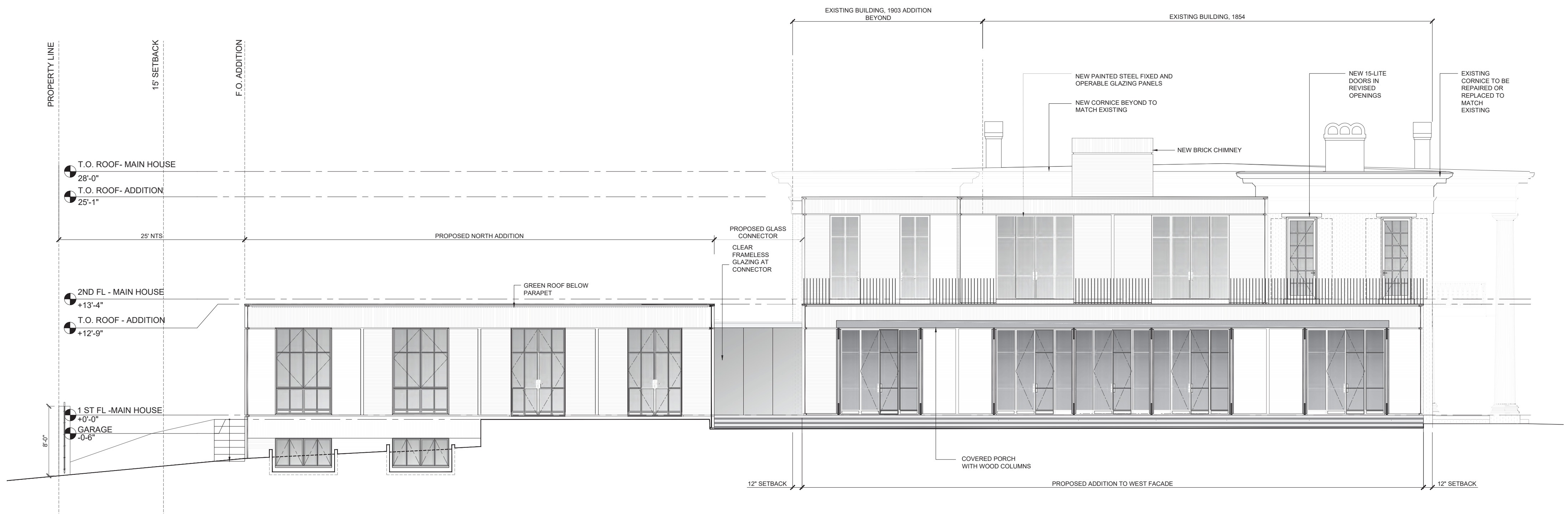
FIGURE B. PROPOSED WEST ELEVATION
