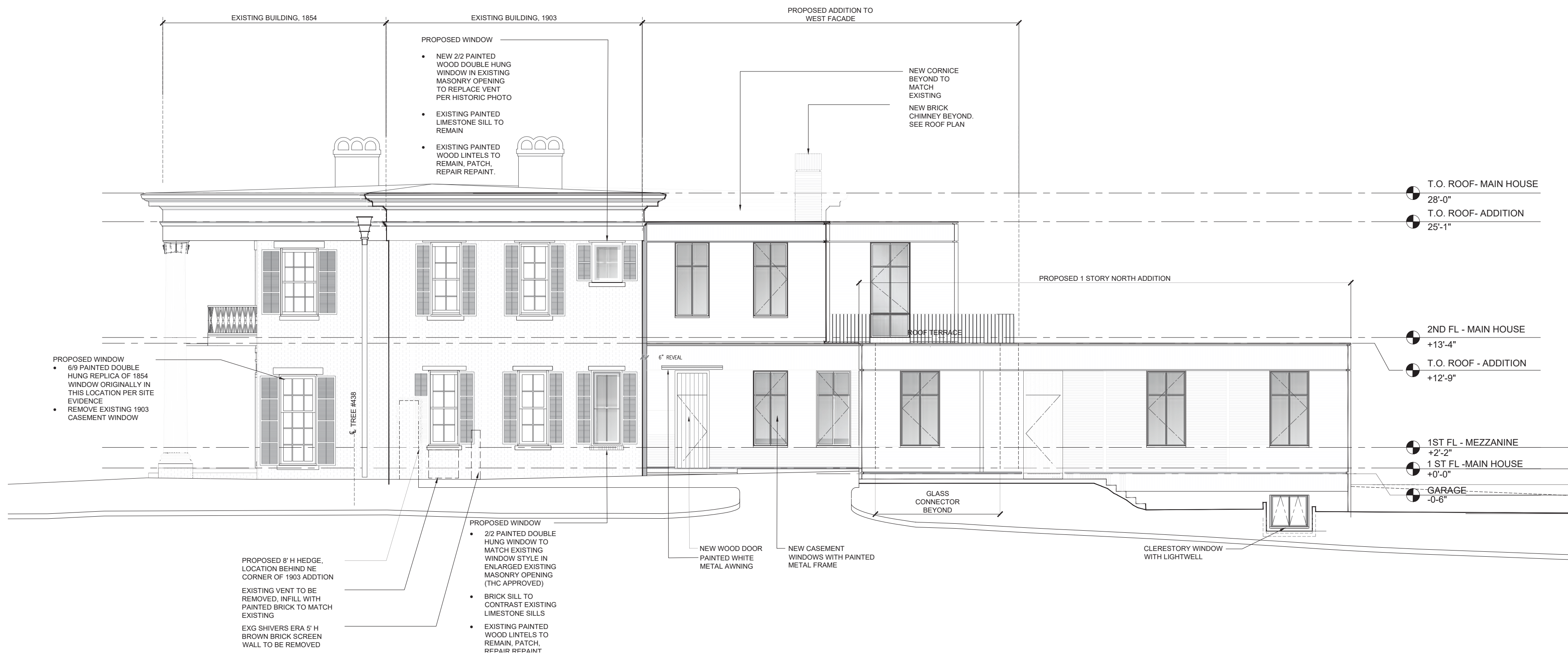
FIGURE B. PROPOSED NORTH ELEVATION
