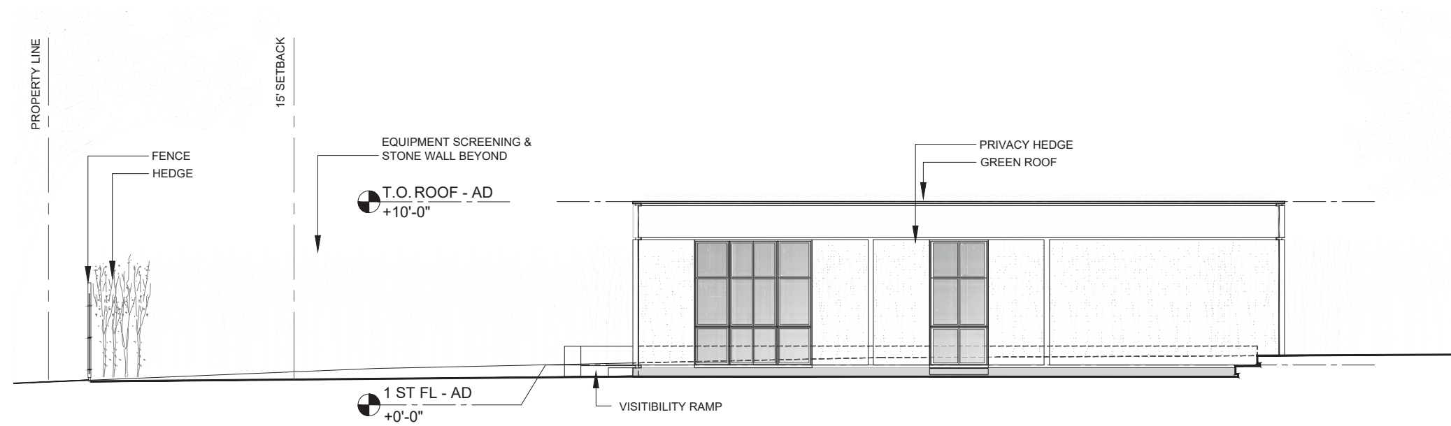
EAST ELEVATION
