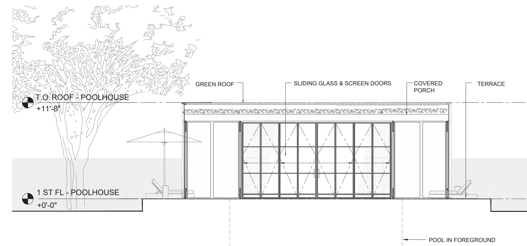
EAST ELEVATION 1/8"=1'0"
