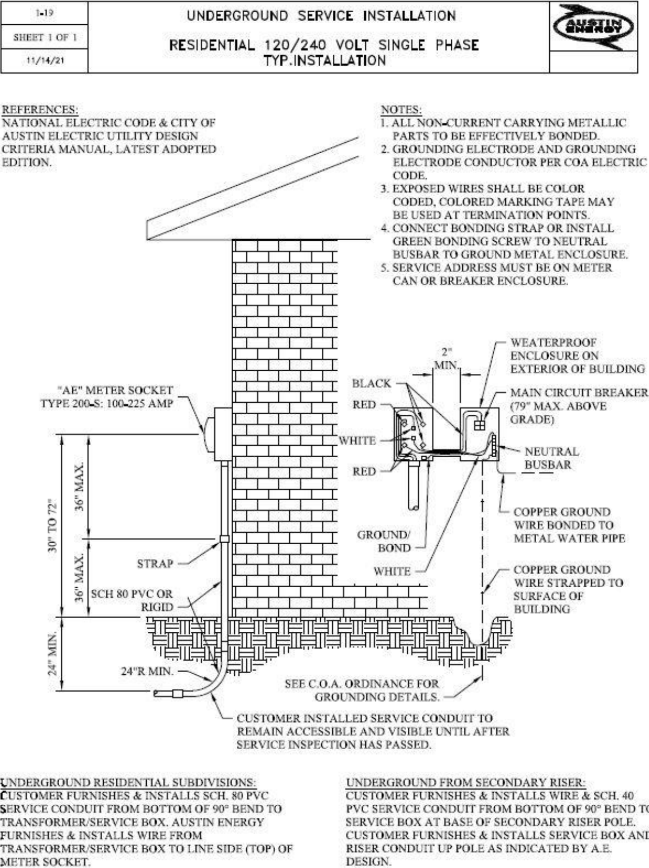
Figure 1-19. Underground Service Installation (Residential – Typical Installation)
