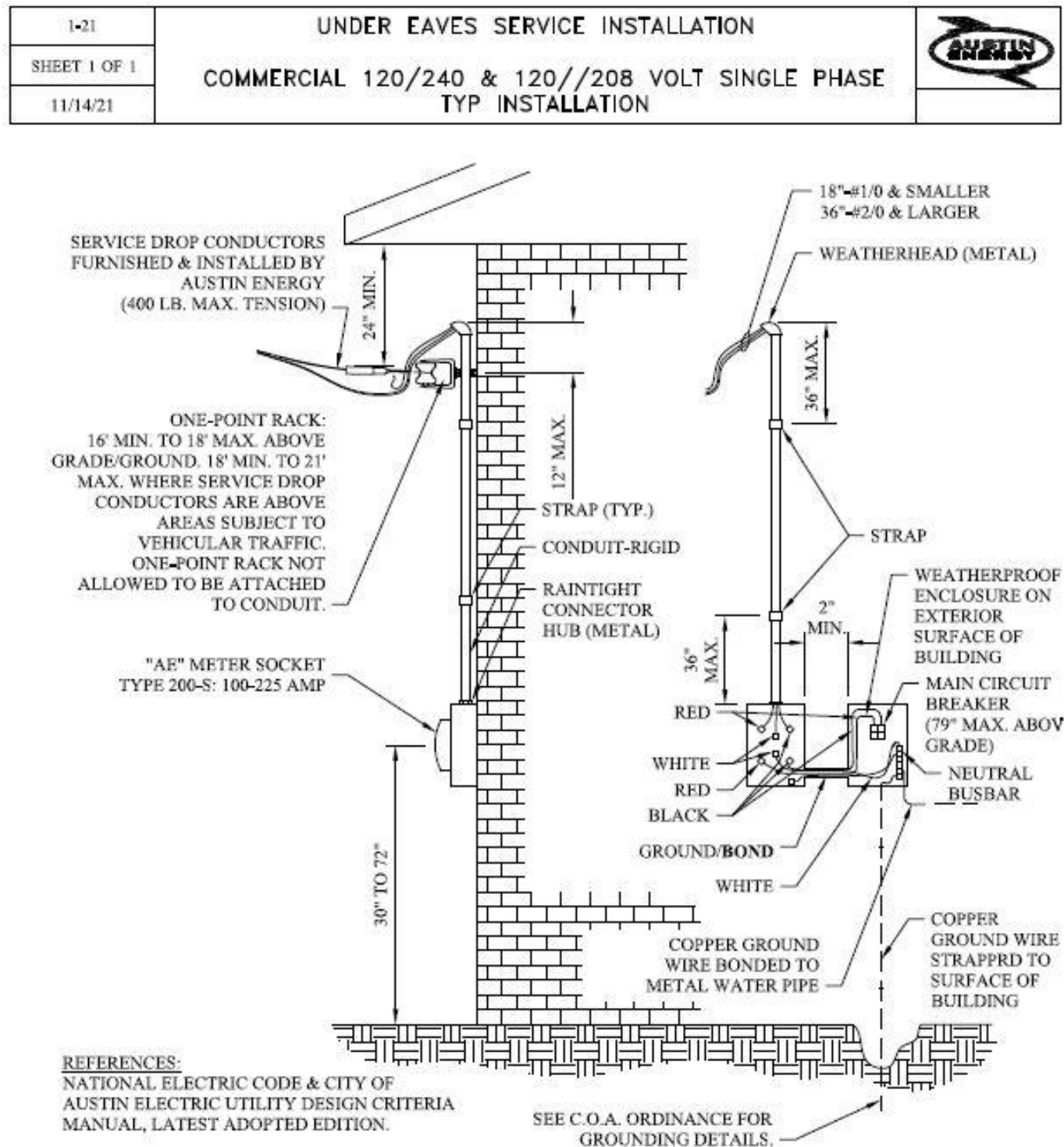
Figure 1-21. Under-Eaves Service Installation (Commercial – Typical Installation)
