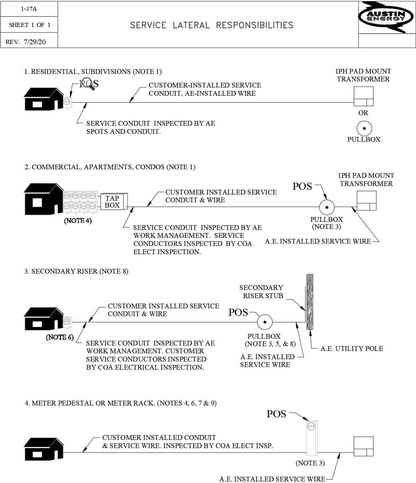
Figure 1-37B Responsibilities from the Point of Service
