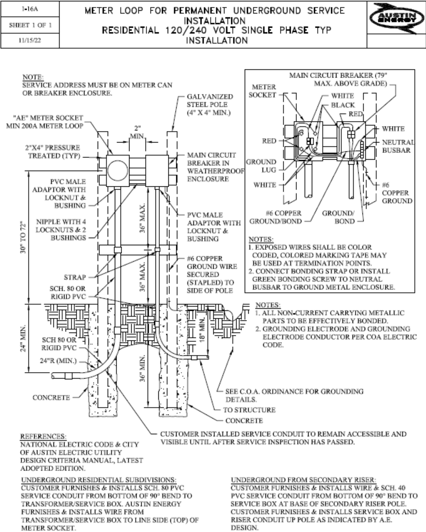
Figure 1-16A. Meter Loop for Permanent Underground Service Installation (Residential/Commercial - Typical Installation)
