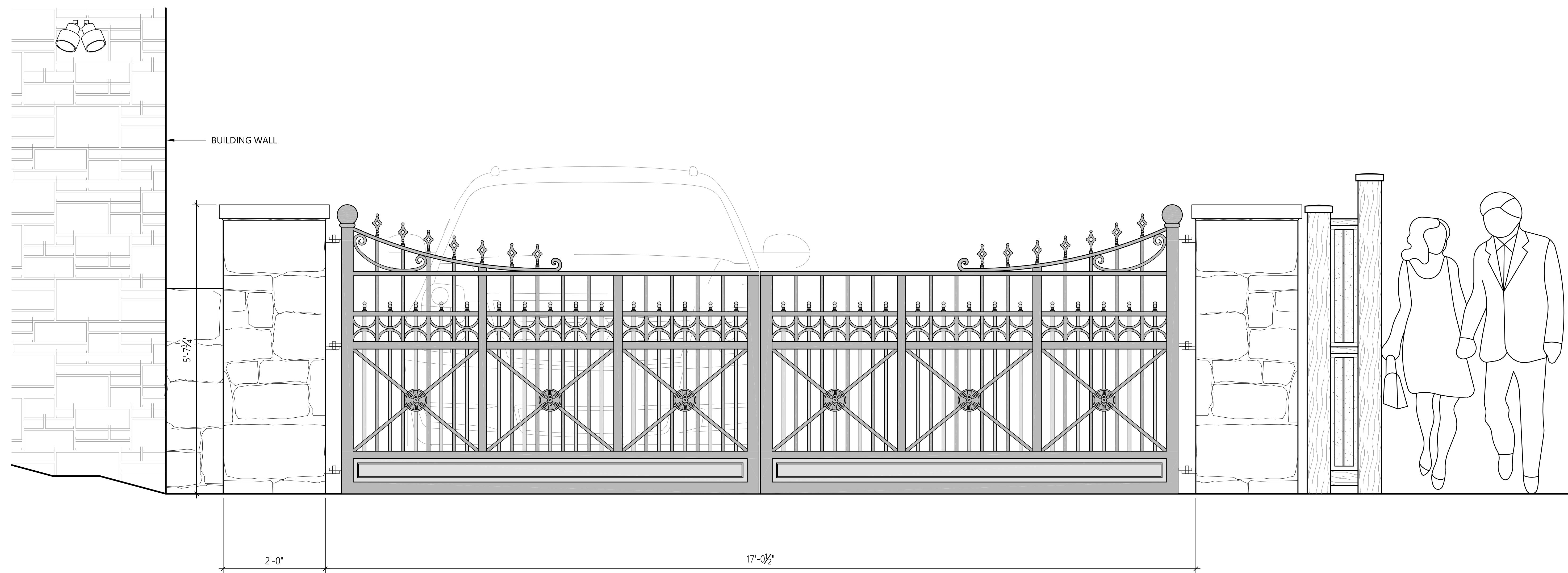
IRON VEHICULAR GATE AT ENTRY
