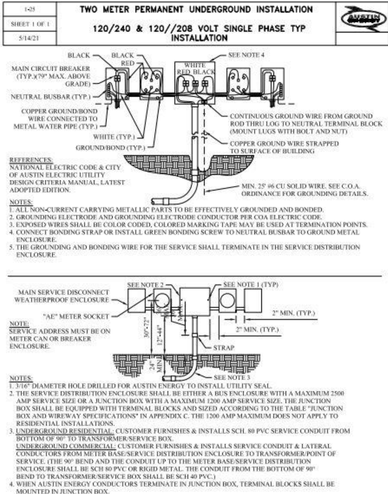
Figure 1-25. Two-Meter Permanent Underground Installation (Typical Installation)
