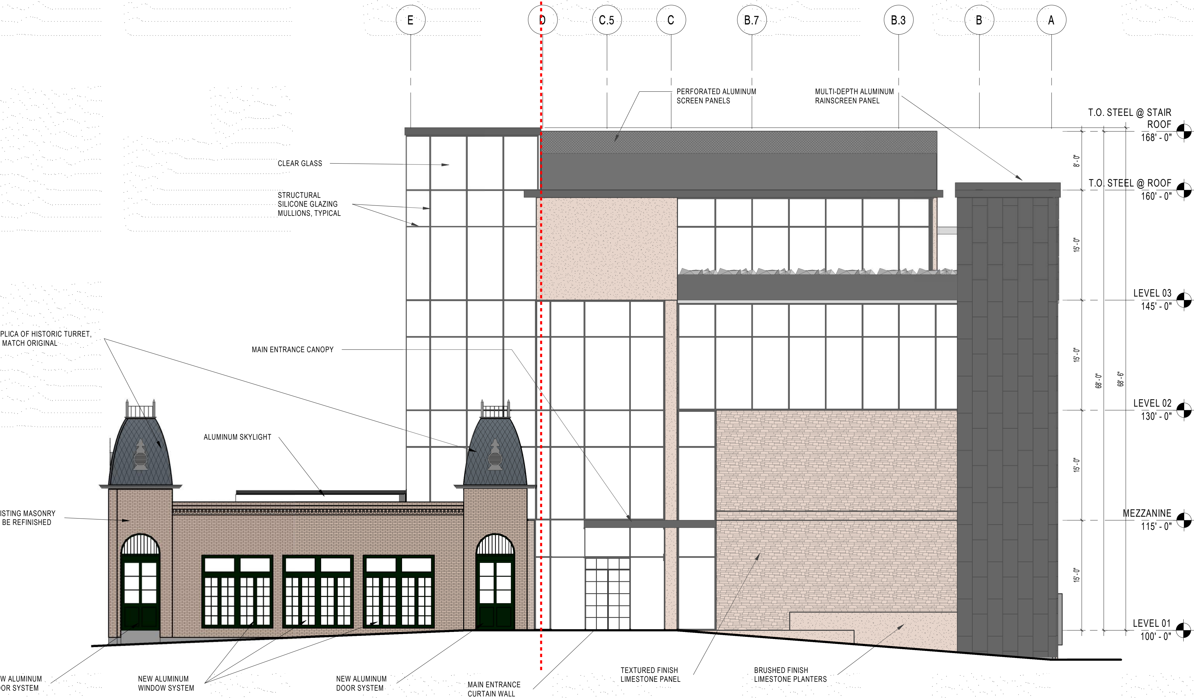
3 | BUILDING ELEVATION - EAST - PRESENTATION A6 | 1/8" = 1'-0"
