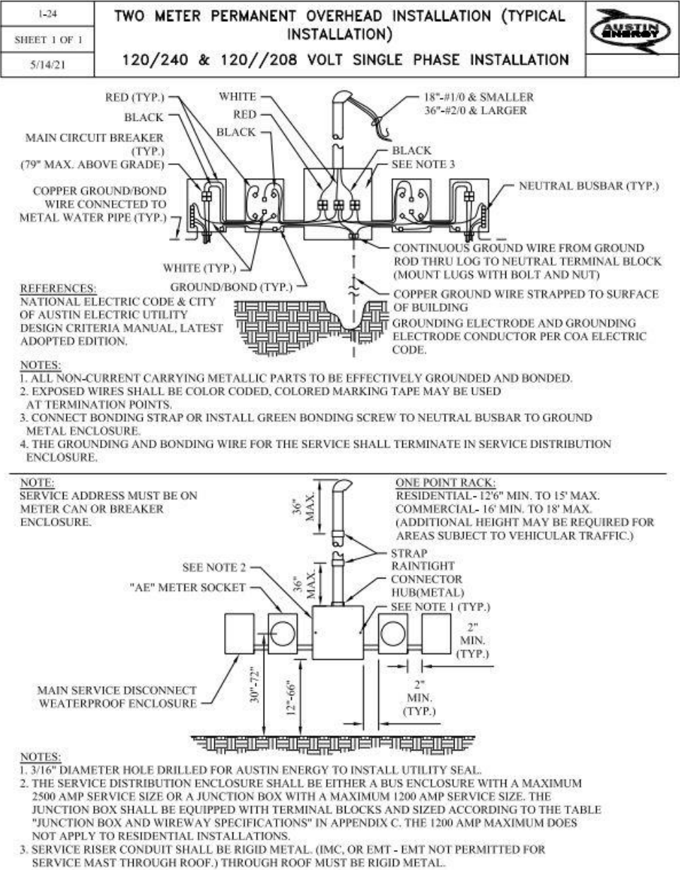
Figure 1-24. Two-Meter Permanent Overhead Installation (Typical Installation)
