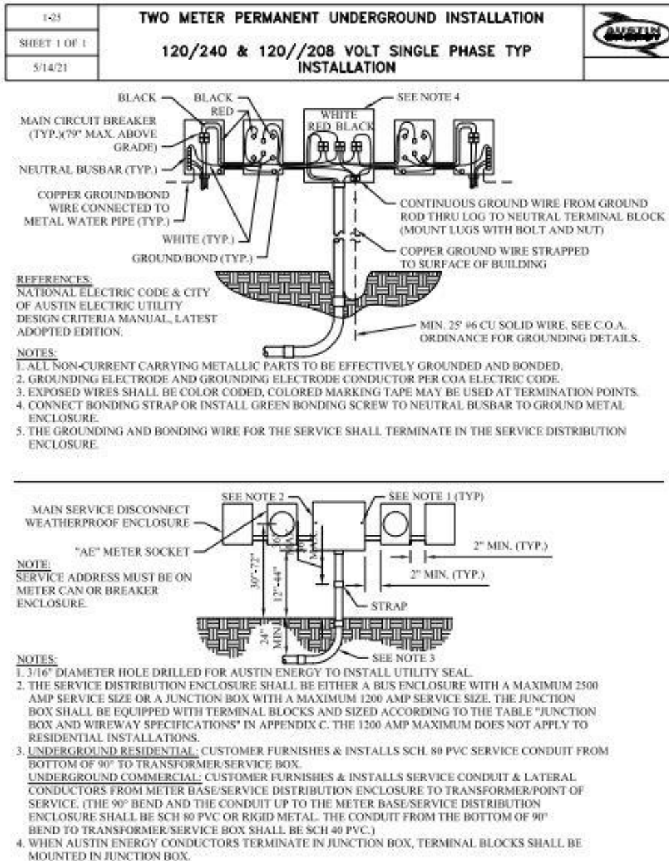
Figure 1-25. Two-Meter Permanent Underground Installation (Typical Installation)
