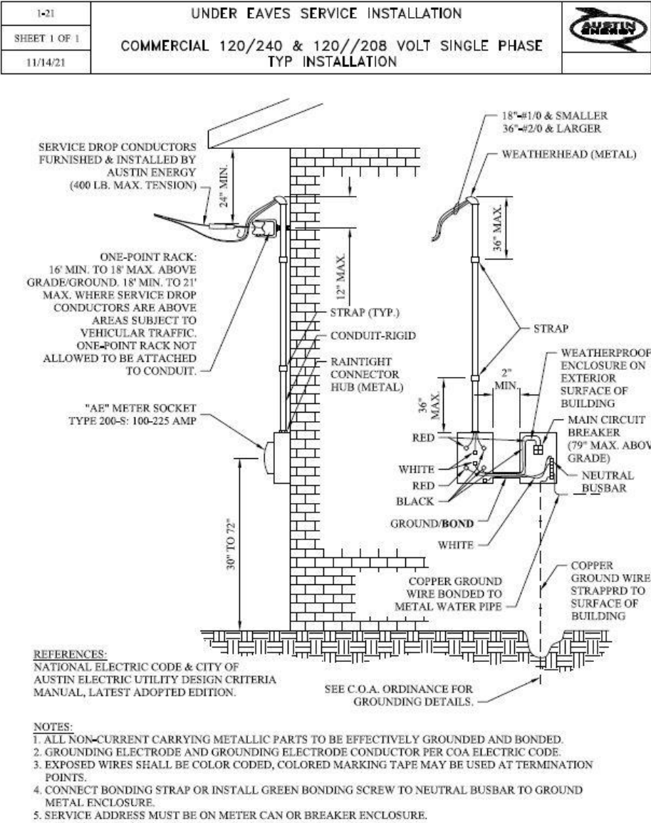
Figure 1-21. Under-Eaves Service Installation (Commercial – Typical Installation)
