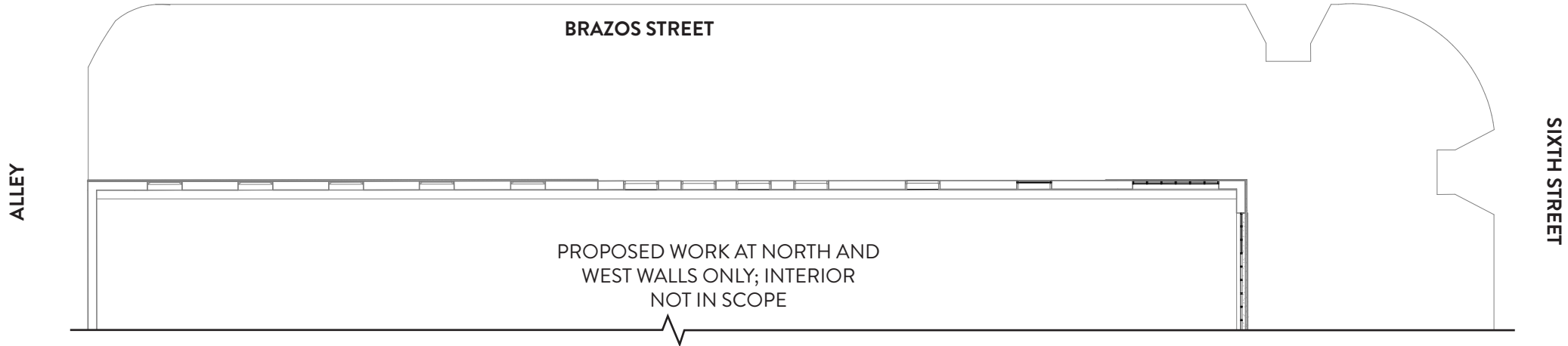
PROPOSED FIRST FLOOR PLAN AT WEST WALL
