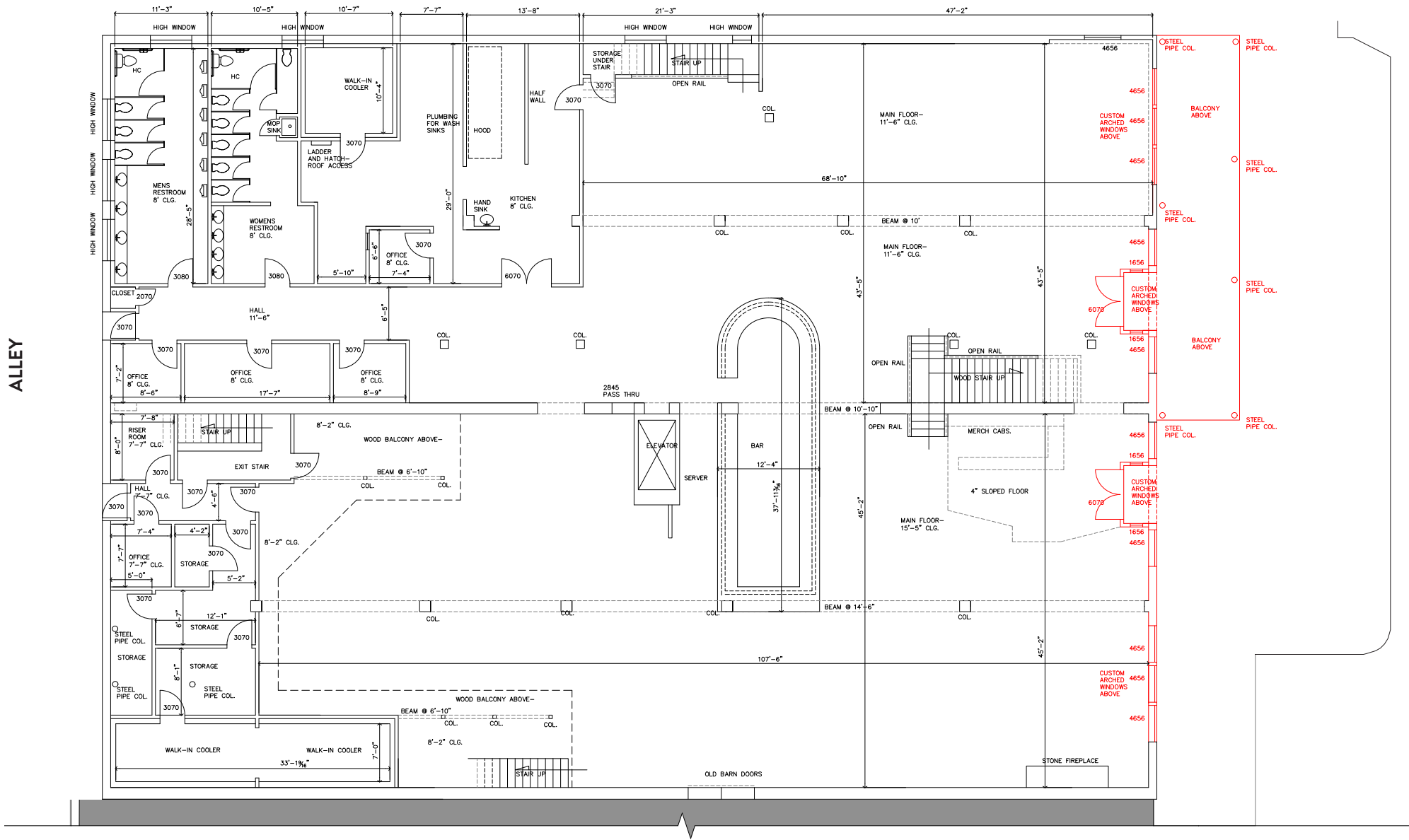
EXISTING FIRST FLOOR PLAN & PROPOSED DEMOLITION
