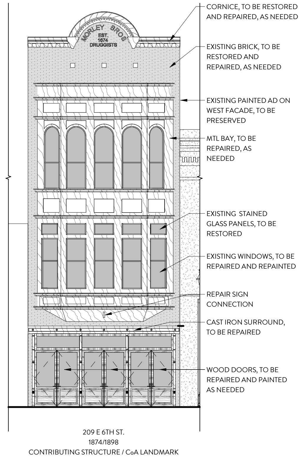
PROPOSED ELEVATION
