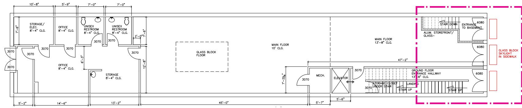
EXISTING FIRST FLOOR PLAN
