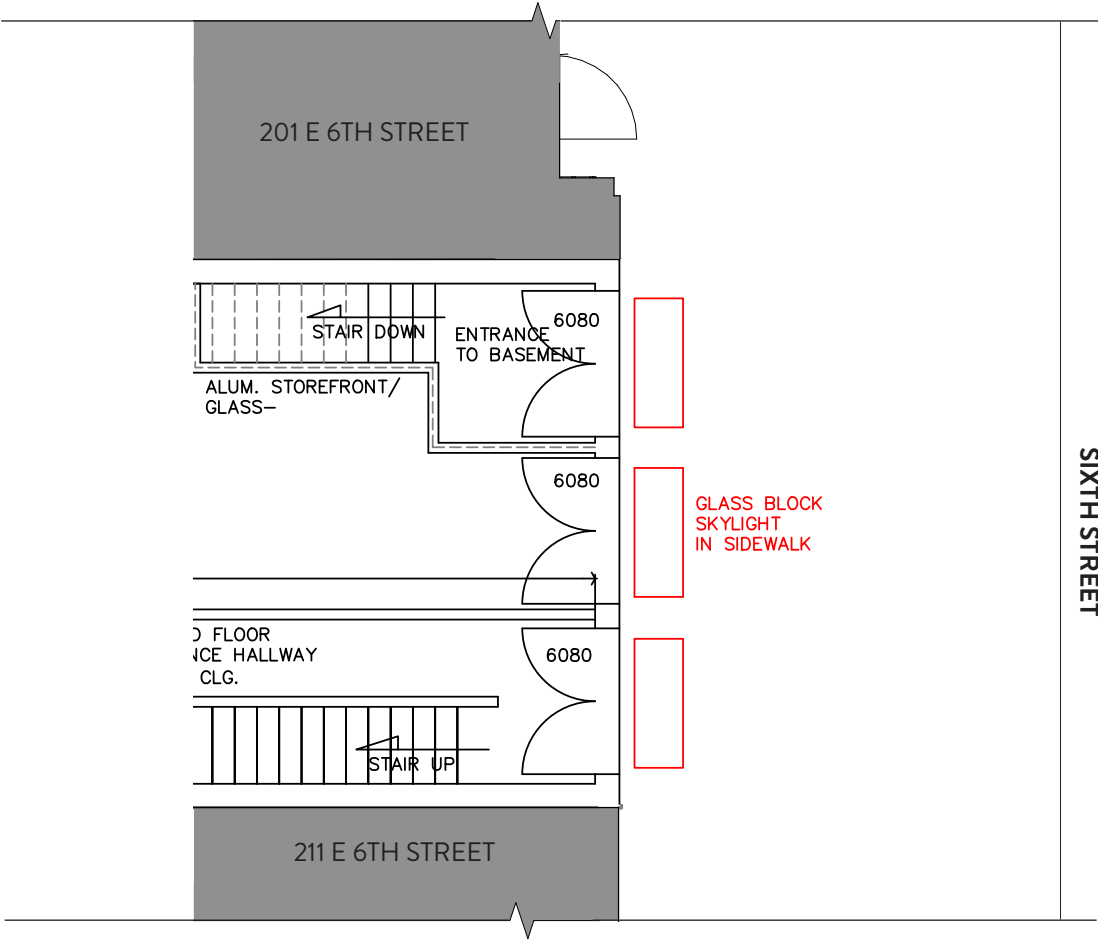
ENLARGED EXISTING FIRST FLOOR PLAN AT NORTH WALL
