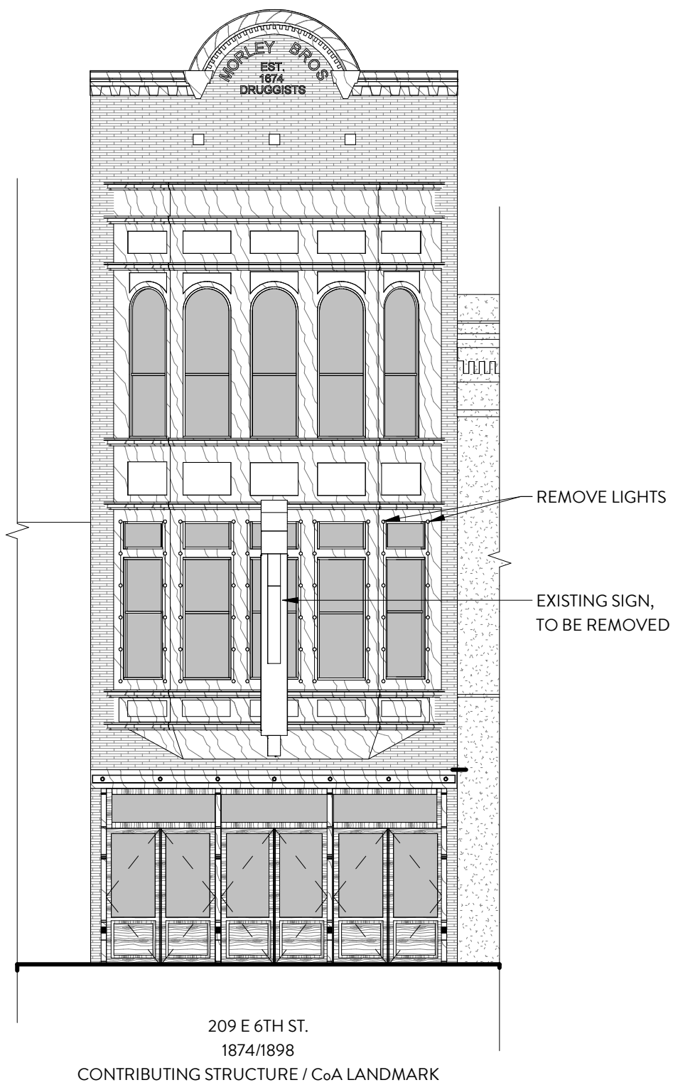
EXISTING ELEVATION
