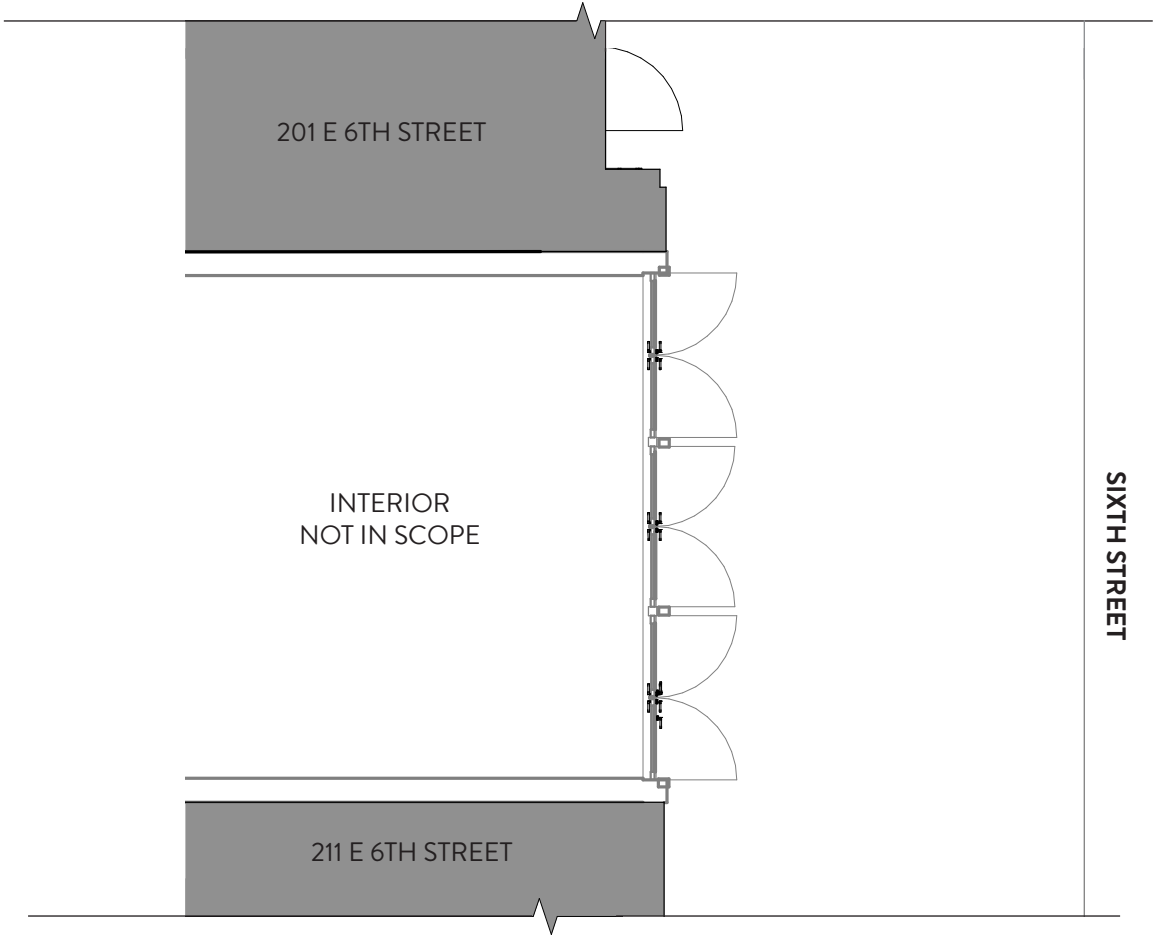
ENLARGED PROPOSED FIRST FLOOR PLAN AT NORTH WALL
