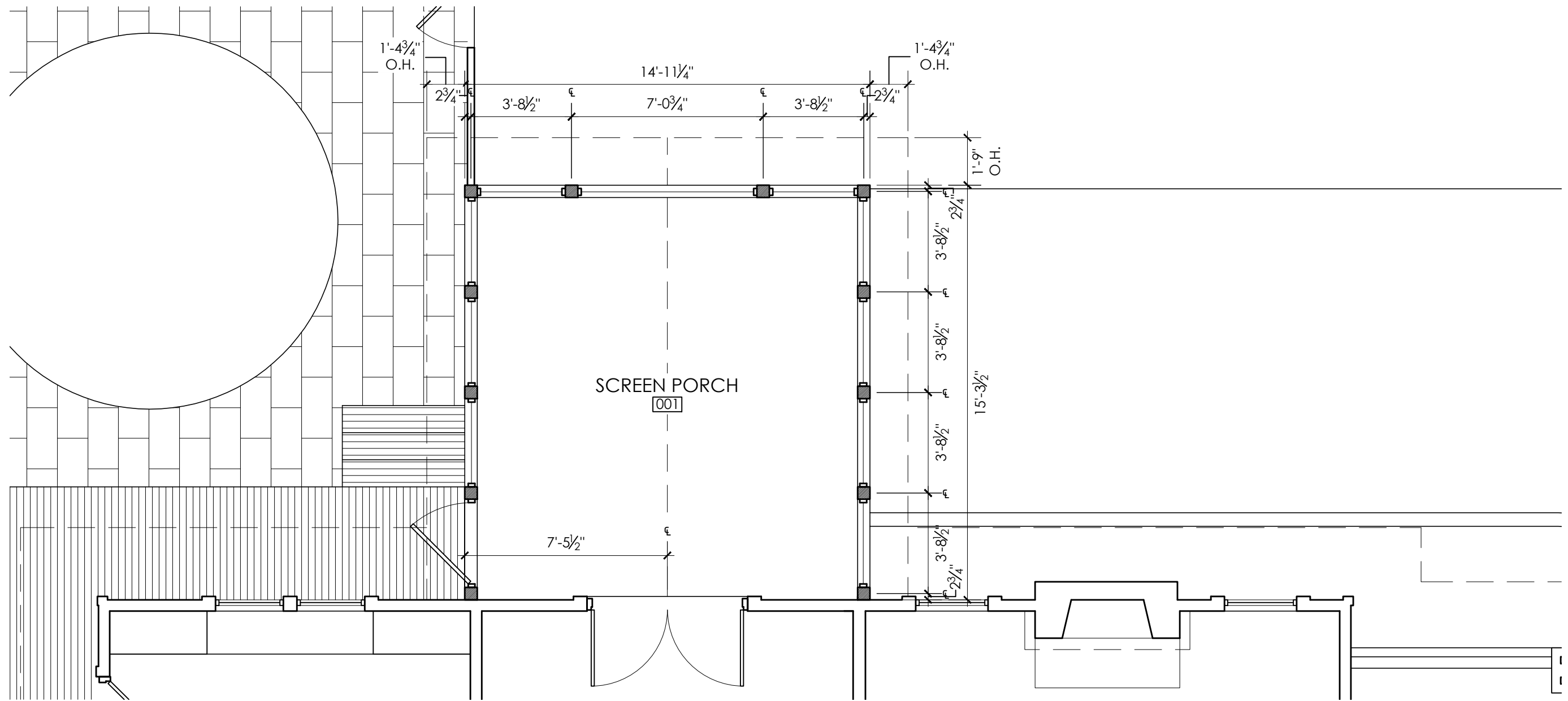
1 SCREEN PORCH FLOOR PLAN 1/4" = 1'-0"
