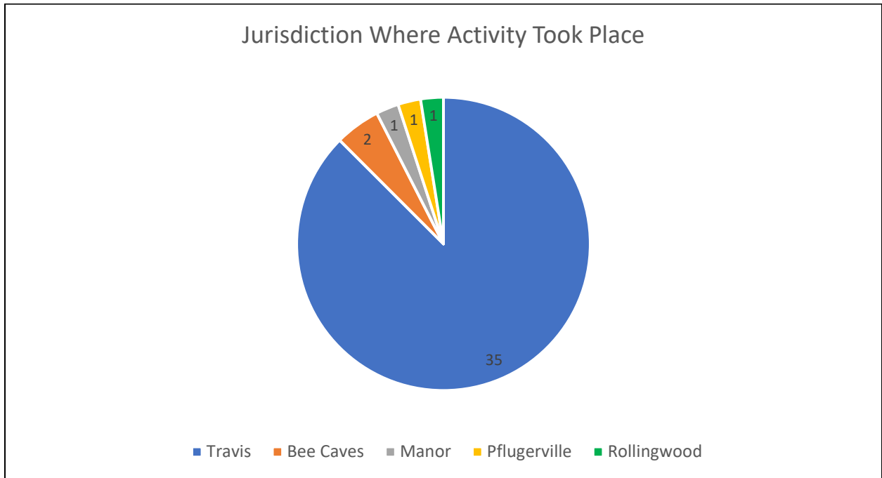
Figure 3. Where wildlife activity was reported based on Jurisdiction within Travis County.
