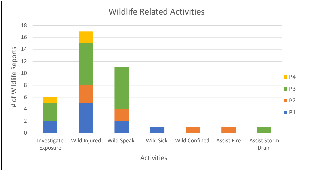
Figure 1. Wildlife Related Activities that took place in Travis County.
