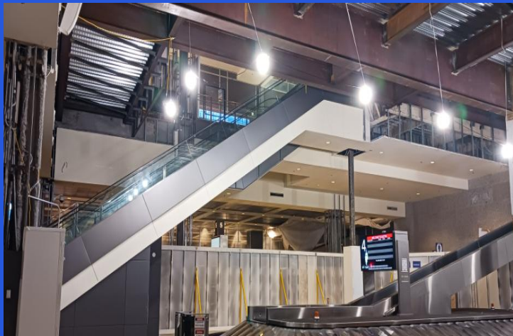
Steel decking Phase 1 complete
